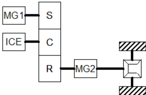
Fig. 9: Hybrid Synergy Drive mechanism
