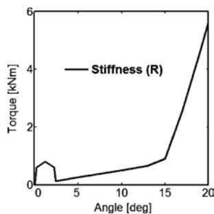
Figure 7 Stiffness function for R.
