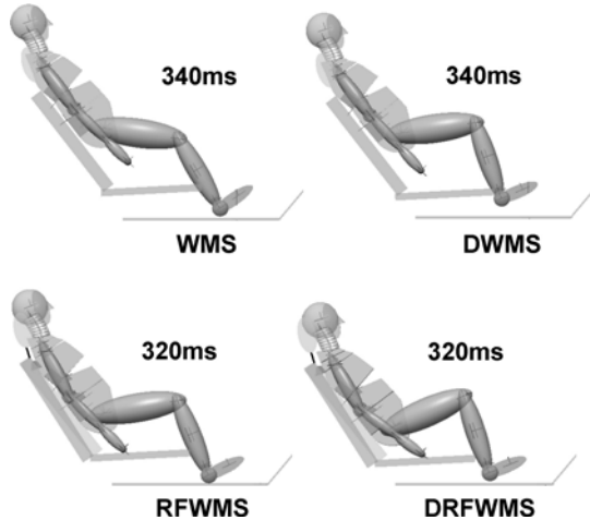
Figure 12 Comparison of the ramping effect of anti-whiplash seat design concepts at the severe crash pulse.
