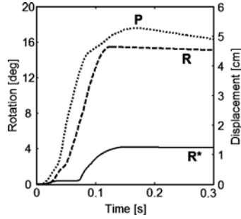
Figure 10 AWD displacements in response to the IIWPG standard pulse.
