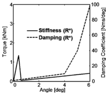
Figure 8 Stiffness and damping functions for R*.
