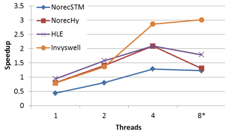
(c) Intruder.
