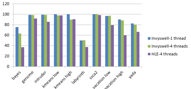
Figure 10: Percentage of Committed Hardware Transactions.
