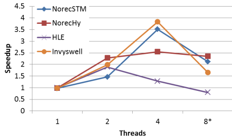
(a) Bayes.
