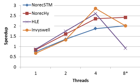
(b) Genome.
