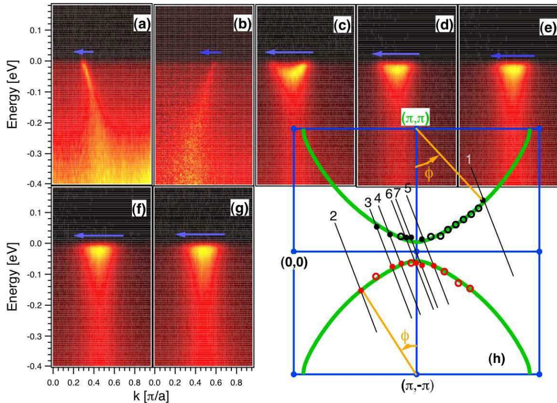
FIG. 1: (Color online) ARPES intensities along momentum cuts that cross the underlying Fermi surface (FS) (a) at the node, (b) to (f) between the node and the antinode, and (g) at the antinode. The corresponding cuts 1 – 7 are indicated in (h). The circles in (h) are the underlying FS determined from our measurements, while the solid line is the FS from a tight-binding fit to our data. The measurements were performed on LSCO ( T_c = 36 K, x = 0.145 ) at 12 K with h\nu = 55 eV.
