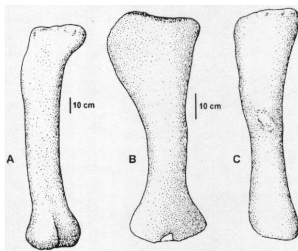
Fig. 15 - Rebbachisaurus tessonei sp. nov. Holotype. Hind limb. A - Left femur in posterior view. B - Right tibia in medial view. C - Left fibula in lateral view. Scale in centimeters.
