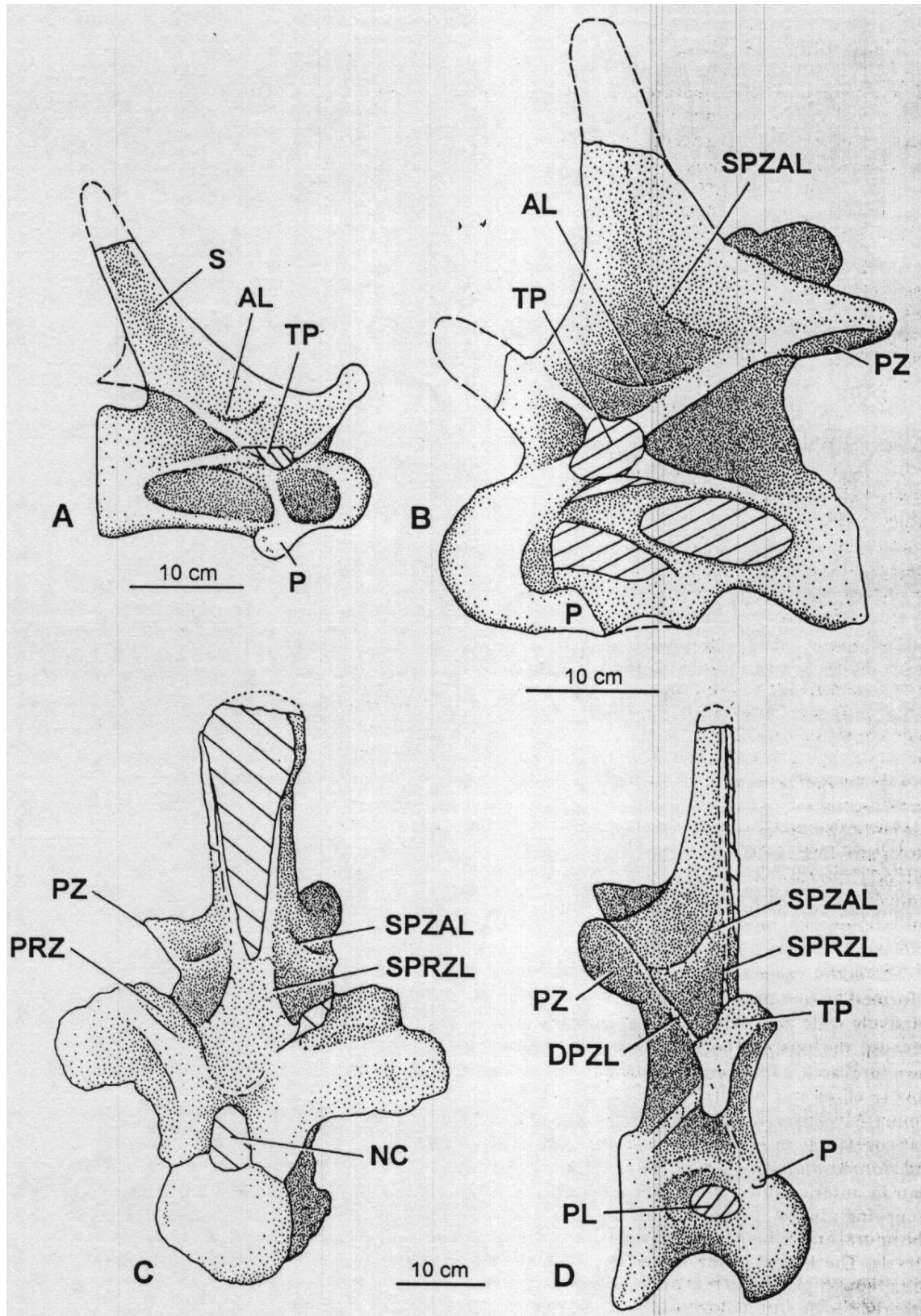
Fig. 8 - Rebbachisaurus tessonei sp. nov. Holotype. Cervical and anterior dorsal vertebra. A - Anterior cervical in lateral view. B - Posterior cervical in lateral view. C, D - Anterior dorsal vertebra in anterior and lateral views. Abbreviations: AL - accessory lamina, DPZL - diapostzygapophyseal lamina, NC - Neural canal, P - parapophysis, PL - pleurocoel, PRZ - prezygapophysis, PZ - postzygapophysis, SPRZL - supraprezygapophyseal lamina, SPZAL - suprapostzygapophyseal accessory lamina, TP - transverse process. Scale in centimeters.
