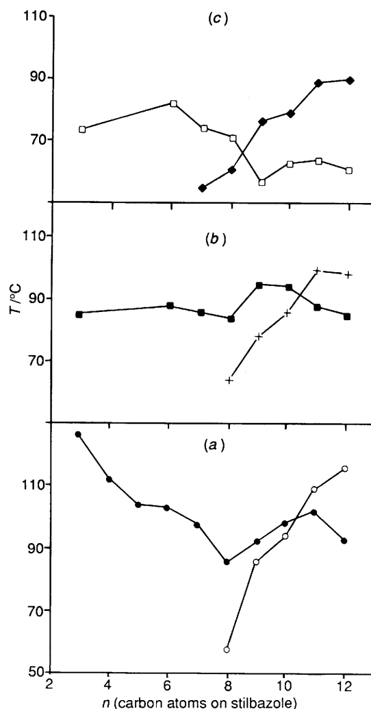
Fig. 2 Phase behaviour of the ethene (a), prop-1-ene (b) and but-1-ene (c) complexes [PtCl 2 (CH 2 =CHC m H 2m+1 )(C n H 2n+1 OC 6 H 4 CH=CH-C 5 H 4 N)] 1 ( m = 0-2 ) as a function of the length of the alkyloxy tail, n , on the stilbazole. Symbols for (a), (b), (c): \bullet , \blacksquare , \square , K \longrightarrow S A , I; \circ , \blacklozenge , S A \longrightarrow I
