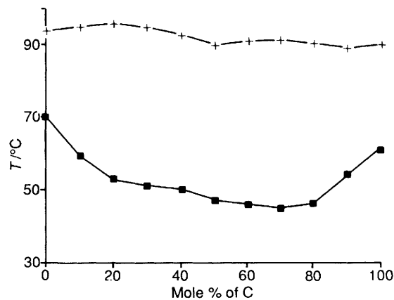
Fig. 6 Phase behaviour of mixtures of the complexes trans -[PtCl 2 -(CH 2 =CHC 3 H 7 )(C 12 H 25 OC 6 H 4 CH=CHC 5 H 4 N)] C and trans -[PtCl 2 -(CH 2 =CHC 6 H 13 )(C 12 H 25 OC 6 H 4 CH=CHC 5 H 4 N)] D: ■, K → S A ; +, S A → I
