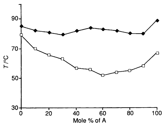
Fig. 5 Phase behaviour of mixtures of the complexes trans -[PtCl 2 -(CH 2 =CHC 5 H 11 )(C 12 H 25 OC 6 H 4 CH=CHC 5 H 4 N)] A and trans -[PtCl 2 -(CH 2 =CHC 5 H 11 )(C 9 H 19 OC 6 H 4 CH=CHC 5 H 4 N)] B: □, K → S A ; ♦, S A → I
