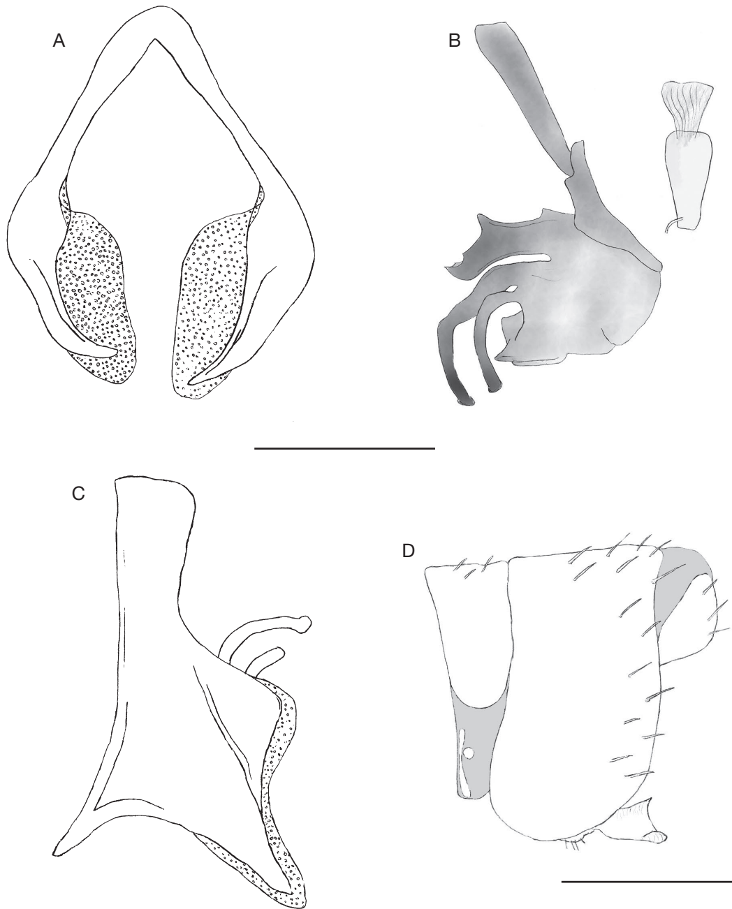
FIG. 5. — Paratype ♂ Thecomyia dideriki Mortelmans n. sp.: A , hypandrium, dorsal view; B , phallopodeme, distiphallus, and acrophalli, lateral view; C , hypopygium, lateral view; D , hypandrium, lateral view. Scale bars: A-C, 0.2 mm; D, 0.4 mm.
