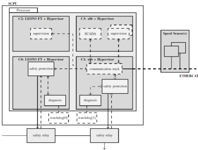
Figure 4: Simplified safety concept (1oo2, multicore).
