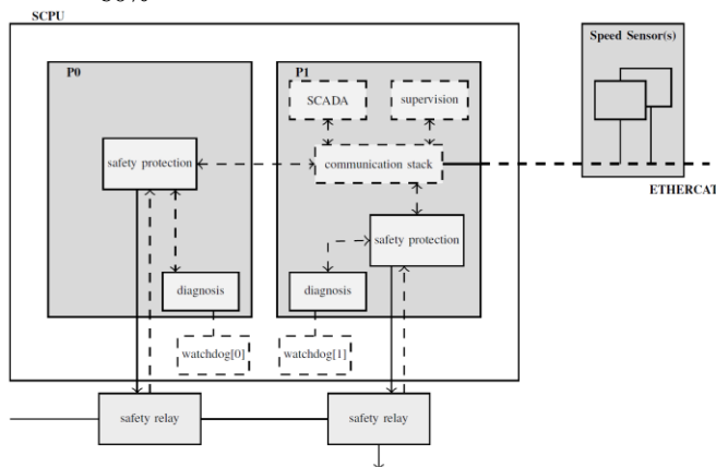
Figure 3: Safety concept (1002; 2 processors)
