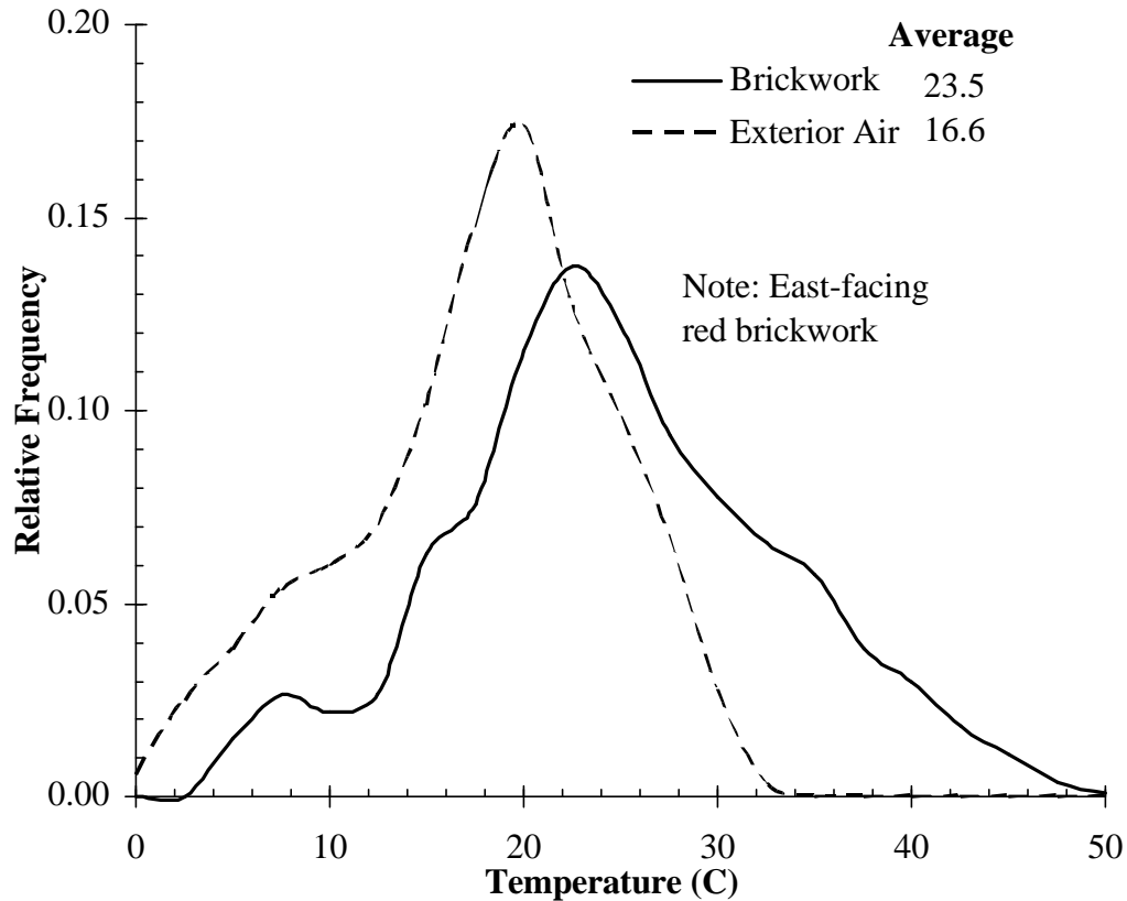
Figure 7: Distribution of Hourly Average Brick Veneer and Exterior Air Temperature over Summer Period
