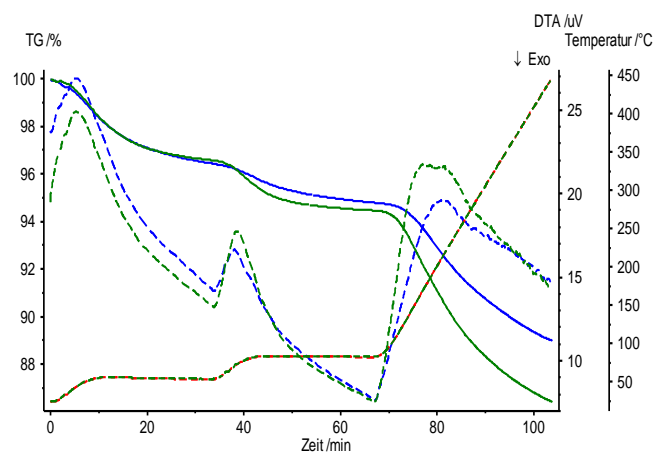
Figure 7 TG (solid lines) and DTA (dashed lines) profiles of two different natural zeolites from Greece: type F (blue, top curve) Type D b (green) upon water saturation at 79% RH.
