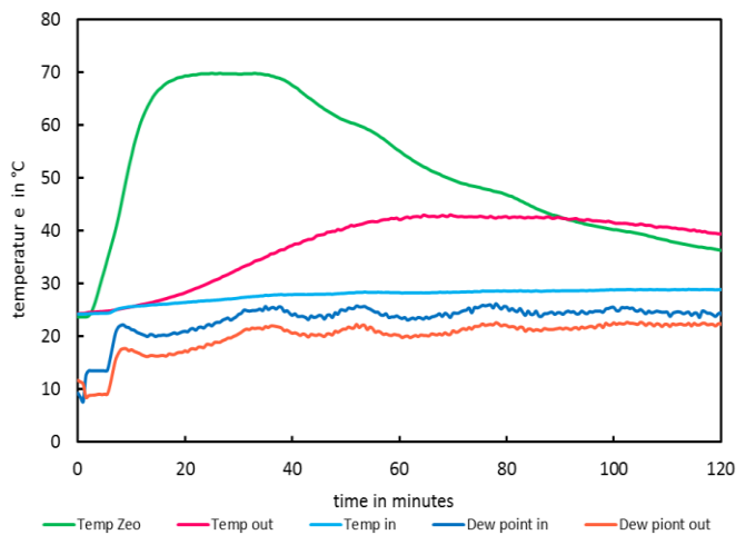
Figure 4 Results of the storage tests (discharging by water adsorption) on the natural zeolitic tuffs from Greece type D b (higher flux).
