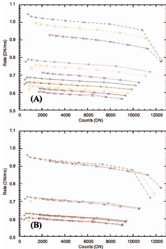
FIG. 68. (Color) The IR spectrometer response rate is calculated using the data shown in Fig. 67 for quadrant A. Plot A shows the subframe imaging modes with a higher response rate. Plot B was created by applying the correction ratios of 0.95 and 0.92 for BINSF1 and BINSF2, respectively. As in Fig. 67, imaging modes are identified by color, and the month of the event is defined by linestyle. The nonlinearity in the IR response becomes more apparent in these curves.
