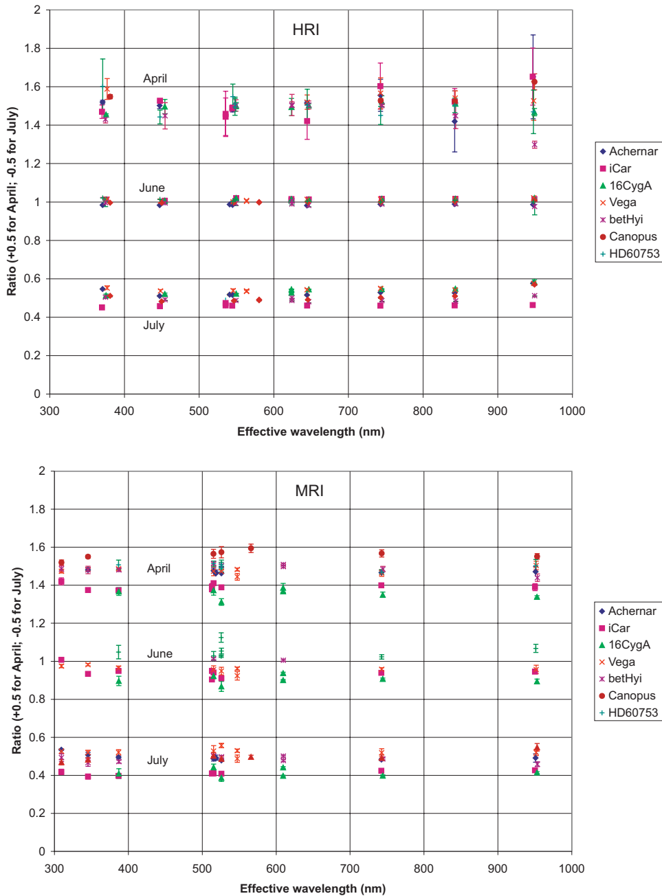
FIG. 28. (Color) Camera response during inflight star calibrations ratioed to those obtained in May 2005 (HRI, top; MRI, bottom). When error bars cannot be seen, they are smaller than the data symbol.
