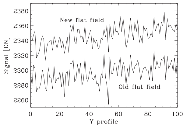
FIG. 37. Comparison of the profile of a coma image with the new flat field including the stimulator pixel-to-pixel relative-response variations and the TV4 flat field.
