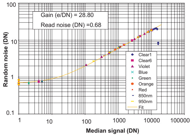
FIG. 23. (Color) Photon transfer data for HRI vis.
