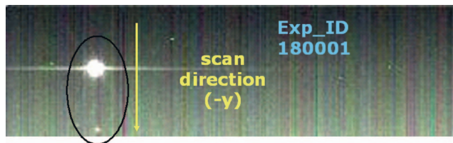
FIG. 98. (Color) Gaussian-stretched, dark-subtracted, composite IR spectrometer image of three bands near 2.1 \mu\text{m} from a scan in the -y direction of the star Canopus. As discussed in the text, a ghost image is clearly detected towards the end of the scan (bottom of image).
