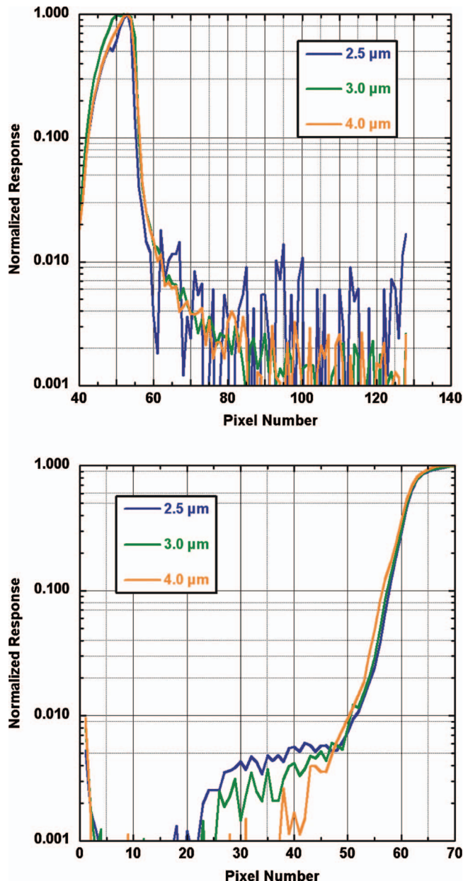
FIG. 97. (Color) Horizontal (top) and vertical (bottom) IR spectrometer profiles of scattered light off the lunar limb (see arrows in Fig. 96). Scattered light levels of 1% are detected 10 pixels from the limb in the horizontal direction and of 2% at 10 pixels from the limb in the vertical direction. The scattered light profiles at all three wavelengths (2.5, 3.0, and 4.0 \mu\text{m} ) behave similarly.
