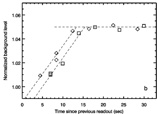
FIG. 75. Normalized IR spectrometer background level as a function of the intersequence gap for the first image in a sequence in mode 1. (a) The full range of observations showing a constant overshoot level (dashed line) for longer gaps. (b) Blowup of the first 33 s, showing the linear rise with intersequence gap time. The diamonds are measurements obtained for mode change from 2 to 1, and the squares are for no mode change (1-1). Linear fits to the rising portion in each of the two cases, indicated by the dashed lines, have the same slope but are offset in time.
