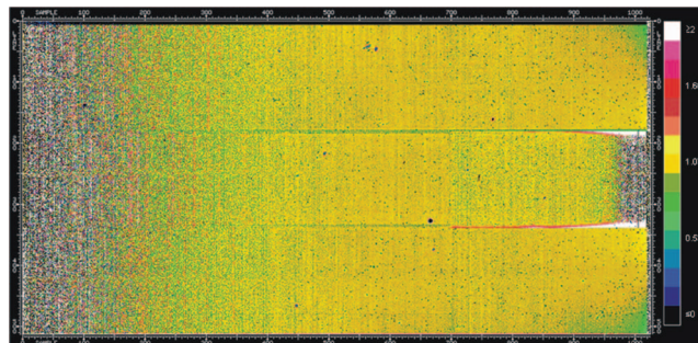
FIG. 91. (Color) Flat-field IR spectrometer image obtained from the L+23 days lunar scan in mode 4; brightnesses are normalized to the mean value. Compared to the TV4 W-lamp/ZnSe window flat, there is almost no structure found in the long-wavelength (rightmost) regions. The horizontal green/red lines are at the boundaries of the central region of the array that is inside the antisaturation filter; some low-frequency structure is apparent at these boundaries. Low SNR at the shortest wavelengths and the longest wavelengths behind the antisaturation filter limits the usefulness of the flat at wavelengths < 1.7 \mu\text{m} ( < column 475) and > 4.1 \mu\text{m} ( > column 950) behind the antisaturation filter.
