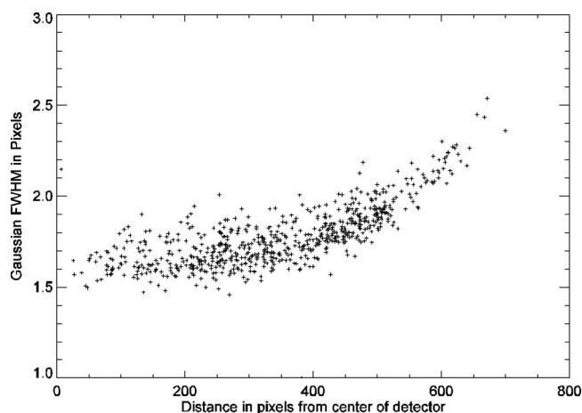
FIG. 16. The PSF FWHM of the MRI after bakeout for 707 stars with peak SNR greater than 100 as a function of distance in pixels from the center of the detector.
