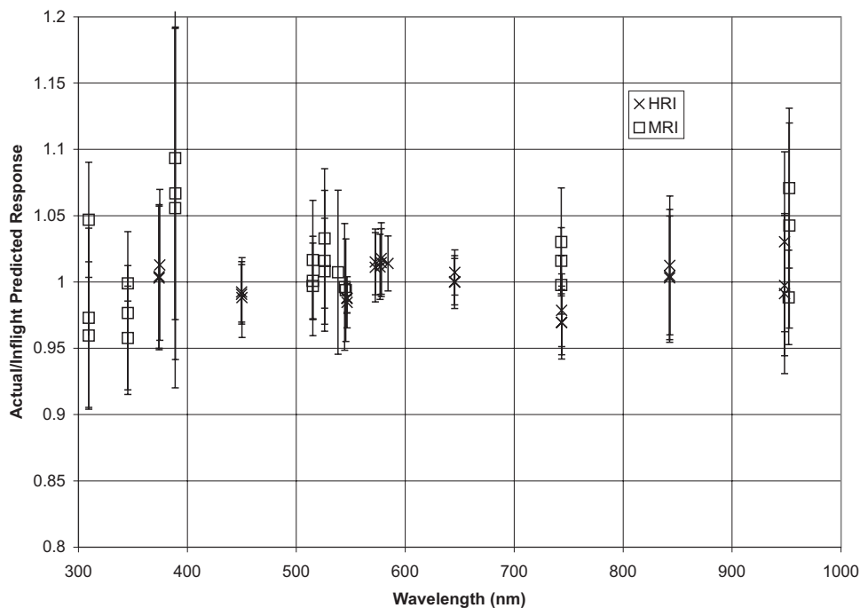
FIG. 30. Ratios of actual inflight stellar response rates to those predicted using the adjusted camera models.
