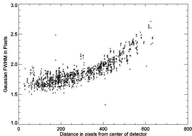
FIG. 15. PSF FWHM in MRI quick alignment images for SNR larger than 100 (1296 stars) as a function of distance in pixels from the center of the detector.
