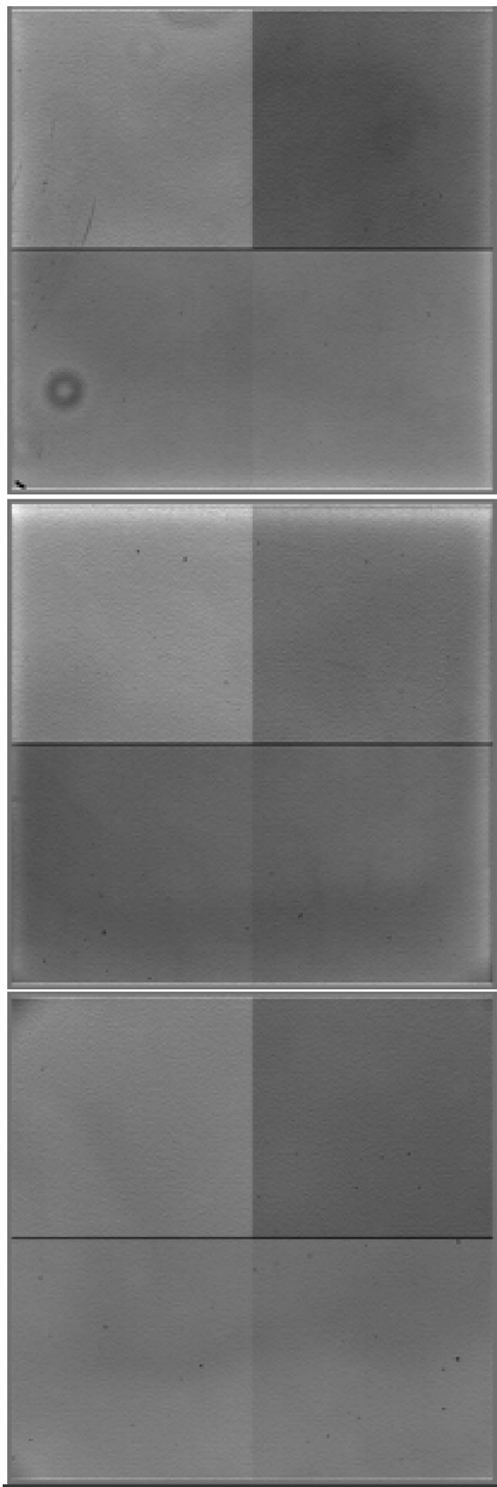
FIG. 34. HRI (top), MRI (middle), and ITS (bottom) flat field for mode 1 and filter 1 (no filter for ITS). Each flat field is a 1024 \times 1024 pixel frame covering all four quadrants. Data span the range from 0.8 (black) to 1.2 (white) in this display with the mean response normalized to 1.0. The upper left quadrant corresponds to quadrant A in the text, the upper right quadrant to B, the lower left quadrant to C, and the lower right quadrant to D.
