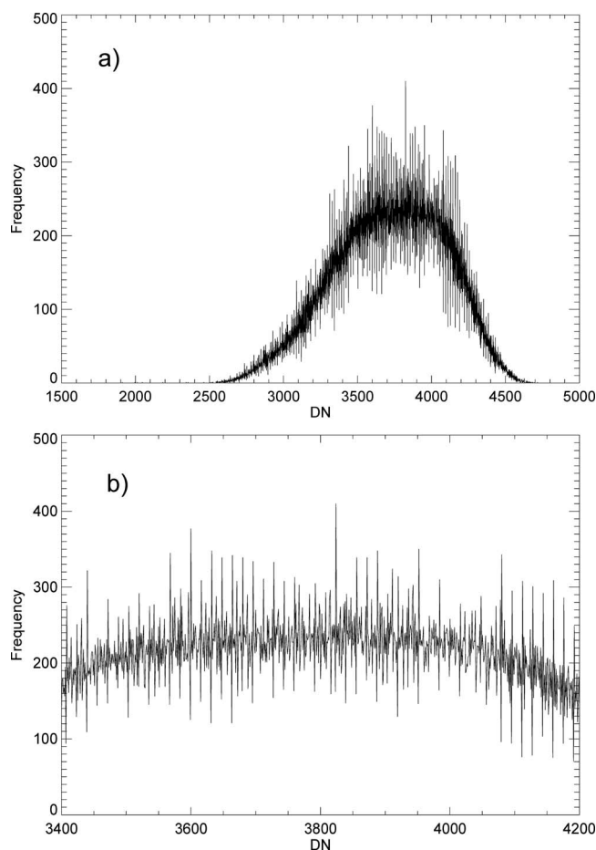
FIG. 40. Histograms of HRI CCD STIM images showing uneven ADC bit weighting: (a) full histogram, (b) expanded view.
