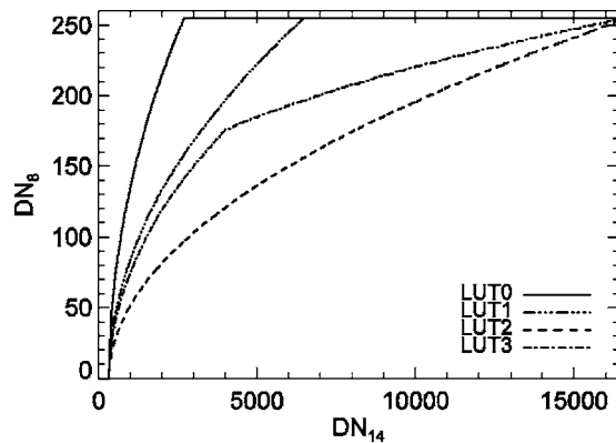
FIG. 102. HRIvis data compression LUT loaded at launch.
