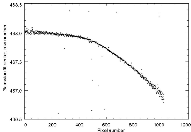
FIG. 62. The inflight variation of the centers of Gaussian fits to the image of the calibration star Beta Hyi as a function of IR spectrometer pixel (column) number. The total variation from one edge of the IR detector to the other is almost exactly one physical pixel.
