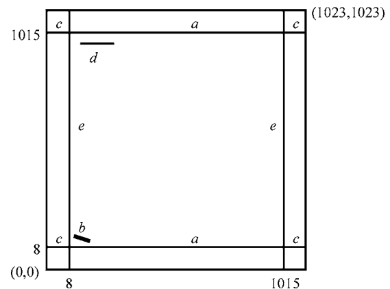
FIG. 33. Bad pixels for HRI, MRI, and ITS in mode 1. The figure is not to scale for illustration purposes. See the text for the definition of marks a–e.
