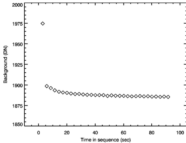
FIG. 74. Background level in a TV2 sequence of 32 IR spectrometer images. The level in the first frame of the sequence is much higher than those in the following images, though subsequent frames continue to drop with time throughout the sequence.
