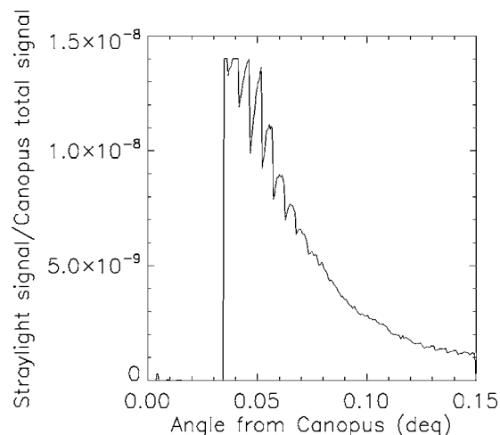
FIG. 44. One of the bright columns from the HRI polar plot in Fig. 43 (at 94^\circ ) normalized with respect to the total Canopus signal showing the worst-case HRI scattered light response to a point source outside the FOV.
