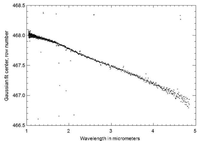
FIG. 63. The inflight variation of the centers of Gaussian fits to the image of the calibration star Beta Hyi as a function of IR spectrometer wavelength. The total center variation in row numbers from minimum to maximum observed wavelength is almost exactly one physical pixel, and the variation is very close to linear with respect to wavelength.
