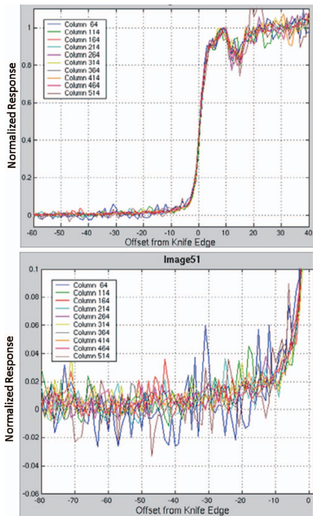
FIG. 95. (Color) IR spectrometer response profiles across a knife edge from the ground-based in-field scattered light test. Signal is detected 10–20 pixels away from the knife edge at a level of 3%–4%. Column numbers represent increasing wavelengths from 1 to 5 \mu\text{m} across the detector. No change in scattered light vs wavelength is seen.
