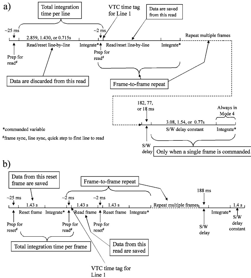
FIG. 6. IR focal plane readout timing. Timing for two different readout modes, (a) interleaved and (b) alternating, are shown.
