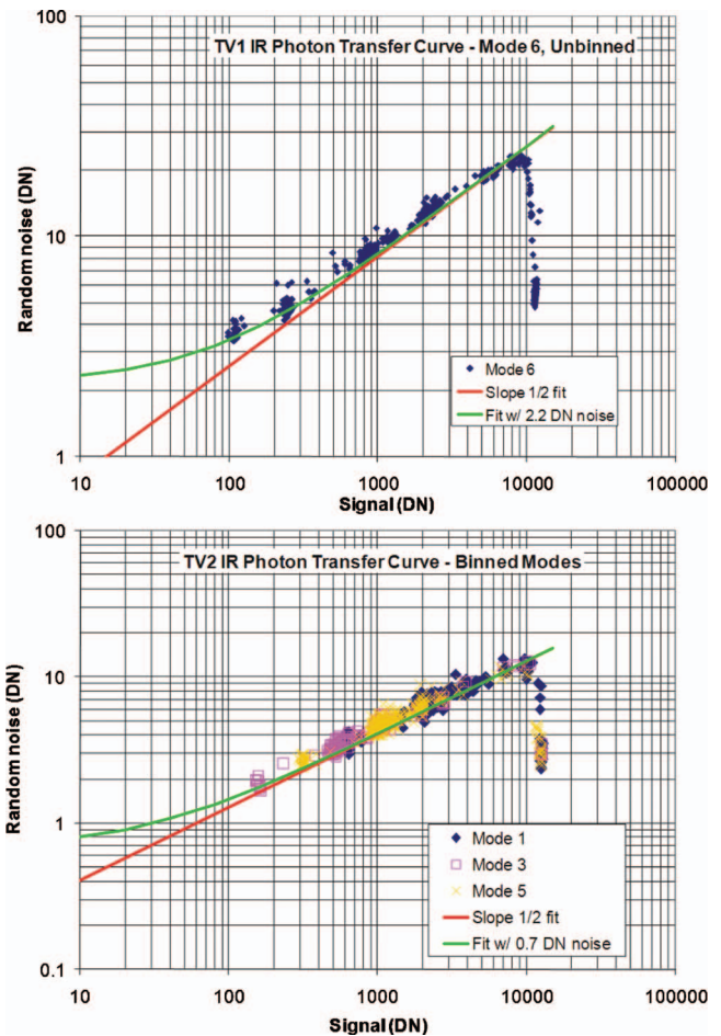
FIG. 70. (Color) IR spectrometer photon transfer data in the unbinned (top) and binned (bottom) modes.
