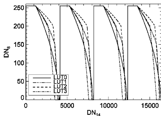
FIG. 105. IR spectrometer data compression LUT loaded on 26 May 2005.
