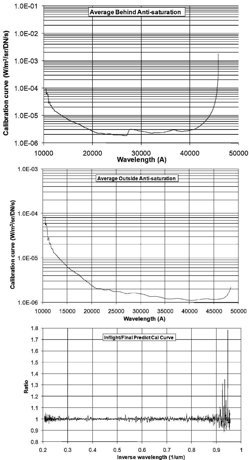
FIG. 85. Best-fit IR spectrometer calibration curves and their ratio to the in-flight measurements.
