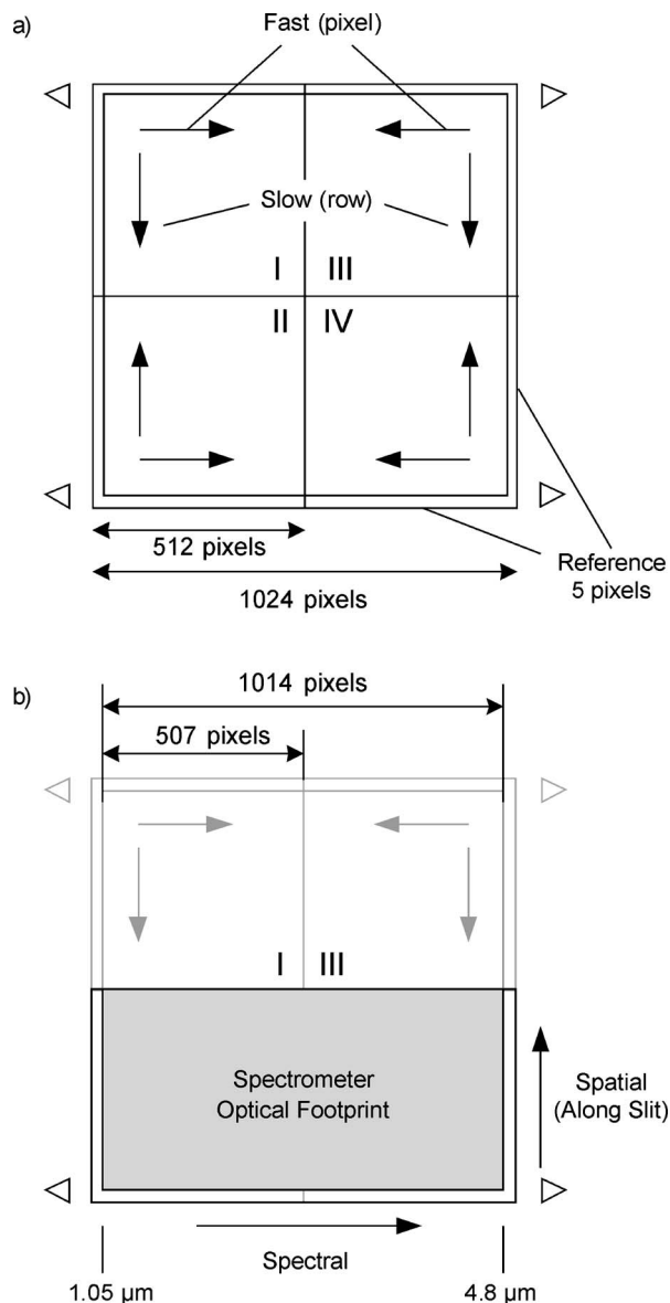
FIG. 5. IR focal plane array architecture (Ref. 3, used with permission). (a) Architecture of the full IR FPA; (b) spectrometer mapping onto the FPA. Only Quads II (A) and IV (B) are used; Quads I and III are not used.
