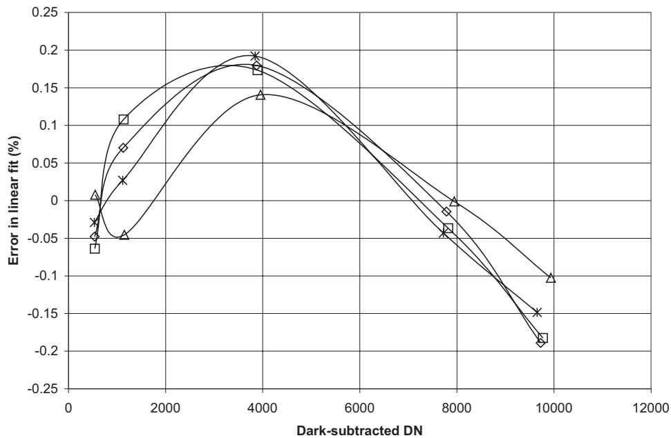
FIG. 22. Residuals to a linear fit of the HRI vis response.
