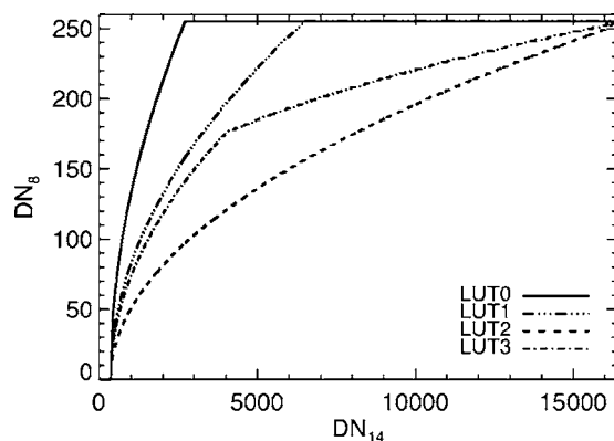
FIG. 12. ITS CCD encounter LUTs for converting 14 bit DN 14 to 8 bit DN 8 s.
