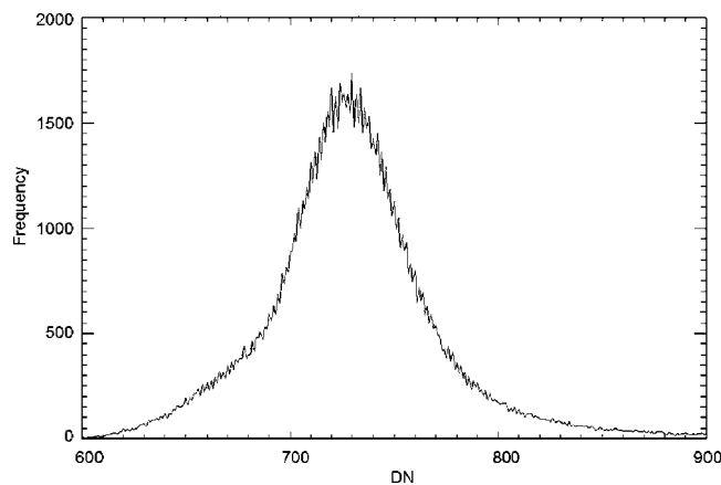
FIG. 94. Histogram of IR spectrometer dark image showing modest uneven ADC bit weighting.
