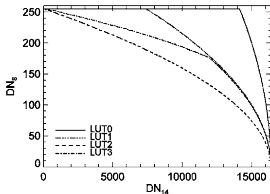
FIG. 104. IR spectrometer data compression LUT loaded at launch.
