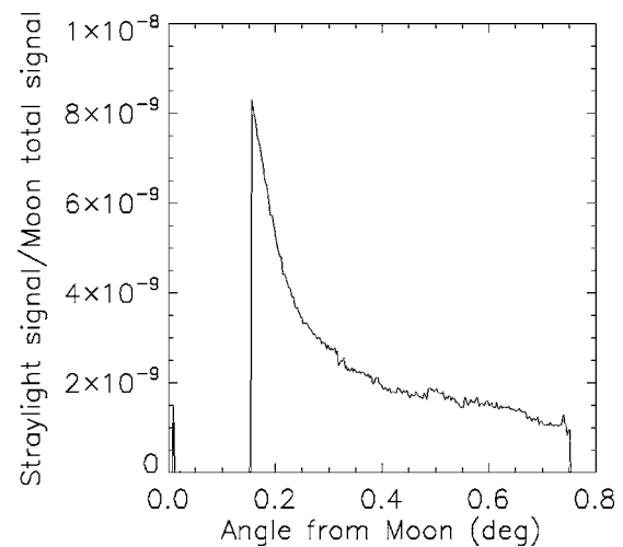
FIG. 47. One of the bright columns from the MRI polar plot in Fig. 46 (at 190^\circ ) normalized with respect to the total lunar signal.
