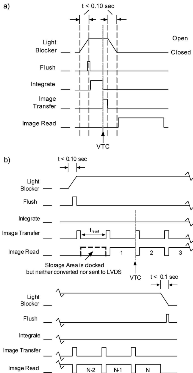
FIG. 4. Generalized timing patterns (Ref. 3, used with permission). (a) Timing pattern for a single exposure when the light blocker is used between each exposure. If N exposures are commanded, then this pattern is repeated N times. (b) Timing pattern when the light blocker is not used between each exposure and there is no additional commanded integration time beyond the minimum. In the second case the number of exposures, N , can be commanded as 1. Both figures show when the time stamp saved in the image header is collected with the arrow and label “VTC.” In both cases the time stamp is collected at the end of the exposure period.
