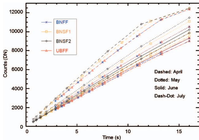
FIG. 67. (Color) The number of IR spectrometer DN measured in the left quadrant A using a resistant mean vs integration time for each imaging mode is shown. Imaging modes are identified by color, and the month of the event is defined by linestyle.
