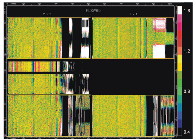
FIG. 88. (Color) Flat-field IR spectrometer images obtained during TV4 with the integrating sphere through the fused-silica window; brightnesses are normalized to the mean value. From top to bottom on the left are modes 5, 3, 2, and 1 flats, and on the right are modes 6 and 4. Wavelength varies from 1 to 5 \mu\text{m} from left to right in each image. The residual vertical structures on the right side of each frame result from regions of minimal input flux to the instrument due to atmospheric and fused-silica window absorptions.
