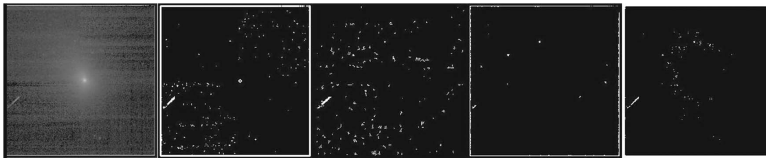
FIG. 53. Calibrated MRI image 6 002 420 ( 256 \times 256 pixels). From left to right: initial image, pixels recognized as CRs by DL_{CRREJ} , CRFIND , IMGCLEAN , and RMCR (at k \text{ lim}=3 and n \text{ limit}=10 ).
