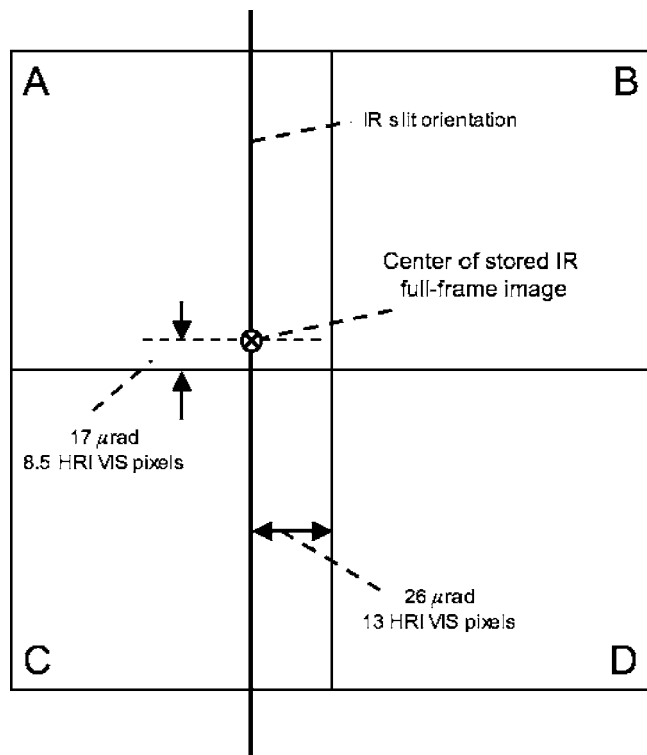
FIG. 57. Relative boresight alignment of the HRI vis and IR spectrometer as measured prelaunch (boresight offsets in figure are not drawn to scale; only the central ~100 pixel subarea of HRI and the central 10% of IR spectrometer slit are shown).
