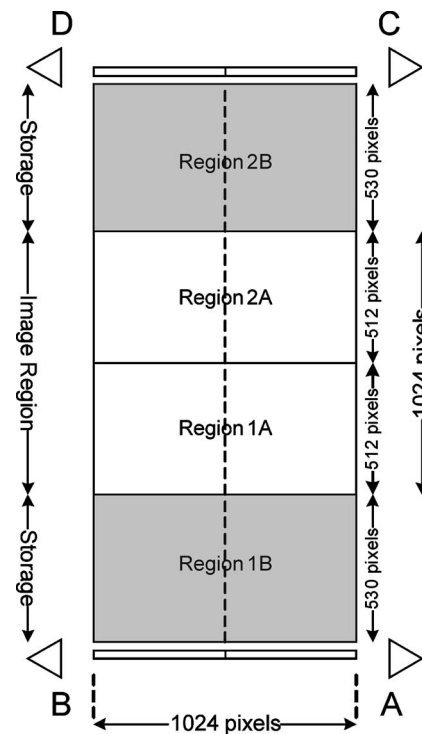
FIG. 3. CCD architecture (Ref. 3, used with permission).
