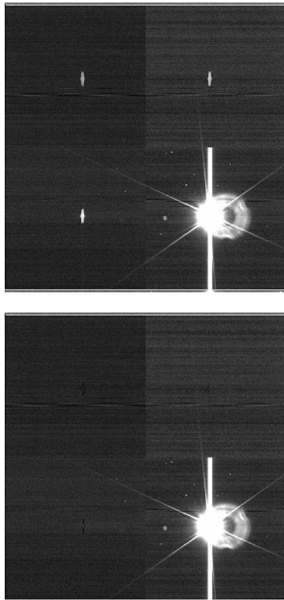
FIG. 41. Saturated image of Canopus before (top) cross-talk correction and after (bottom) cross-talk correction. The electronic ghosts nearly disappear.
