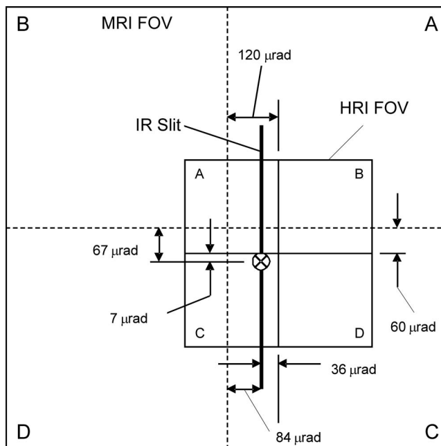
FIG. 58. Relative locations of the HRI-IR slit with respect to the MRI and HRI fields of view measured in flight (boresight offsets in the figure are not drawn to scale; only the central ~250 pixel subarea of HRI, the central ~120 pixel subarea of MRI, and the central 25% of IR spectrometer slit are shown).
