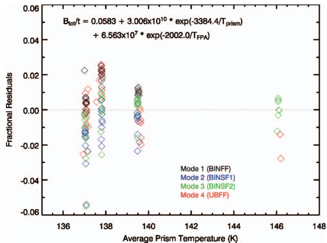
FIG. 73. (Color) Fractional residuals in the background level of inflight IR spectrometer data after the computed FPA dark current and instrument-glow contributions are removed. Residuals for different modes are shown in different colors.
