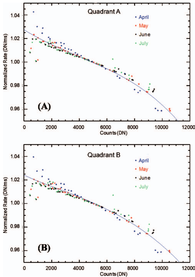
FIG. 69. (Color) The IR spectrometer nonlinearity equations are derived after applying the subframe scaling ratios, and all data are normalized to 1 DN/ms at 5000 DN. Plot A shows the data from quadrant A, and plot B shows the data from quadrant B. Data from each month are represented by a different color.
