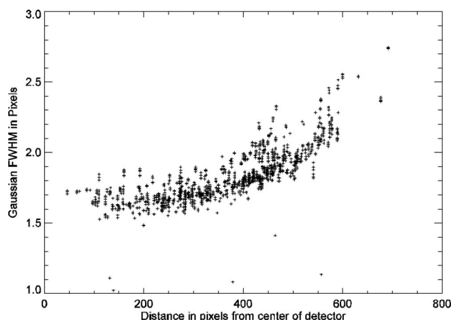
FIG. 17. The PSF FWHM of the ITS from the quick alignment images of 1638 stars with peak SNR greater than 100 as a function of distance in pixels from the center of the detector.
