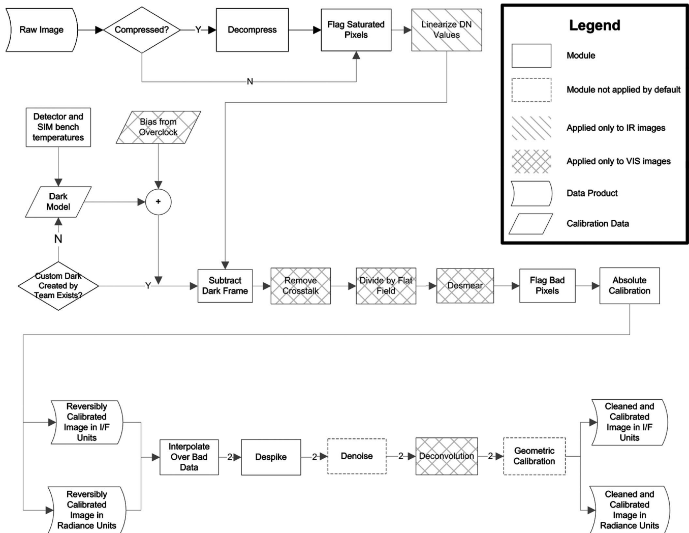
FIG. 101. A flowchart describing the image processing pipeline used to calibrate Deep Impact images. Note that some modules are not applied to all instruments.
