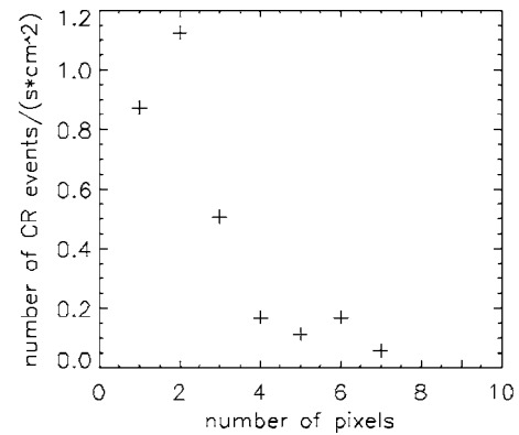
FIG. 100. The number of clusters detected as CR events per \text{s}/\text{cm}^2 vs the number of pixels affected for out-of-peak solar activity in a typical calibrated dark IR spectrometer frame ( 1024 \times 512 ) with t=7.7 s.
