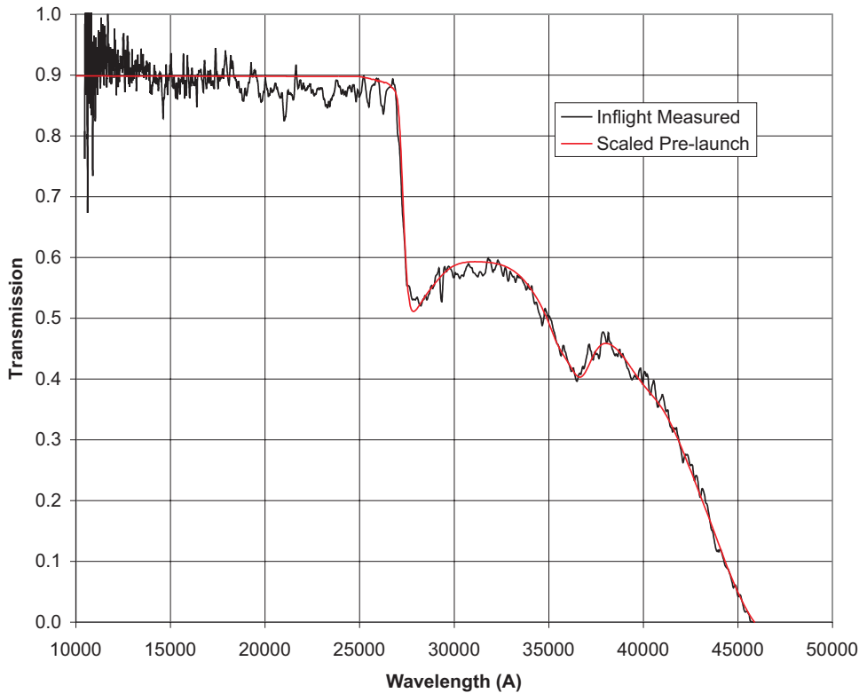
FIG. 83. (Color) IR spectrometer anti-saturation filter spectral transmission curve: black, inflight measurement; red, prelaunch measurement scaled to fit the inflight measurement.
