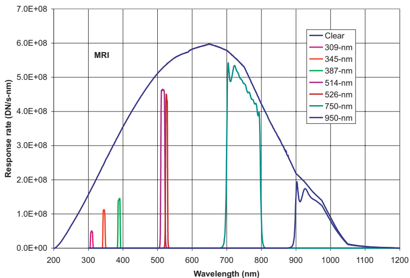
FIG. 31. (Color) Modeled camera response rates to an extended gray source of radiance of 1 \text{ W m}^{-2} \text{ sr}^{-1} \mu\text{m}^{-1} : (a) HRI vis, (b) MRI, and (c) ITS.
