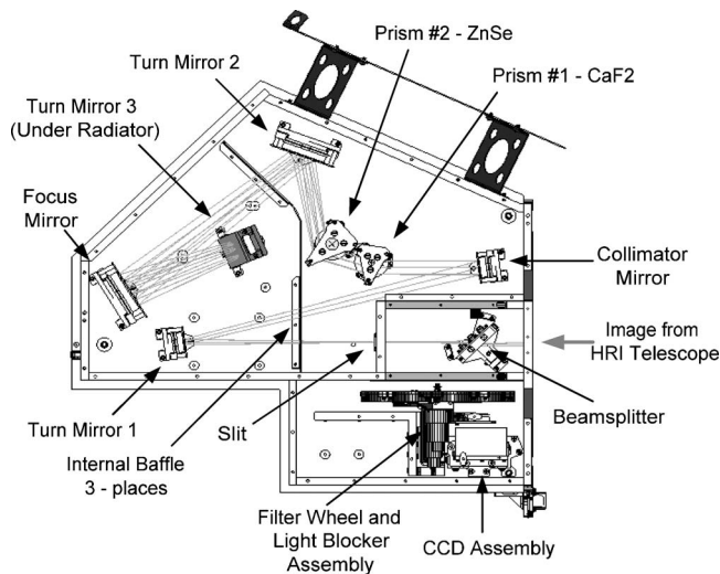
FIG. 56. Detailed layout of the SIM (Ref. 3, used with permission).
