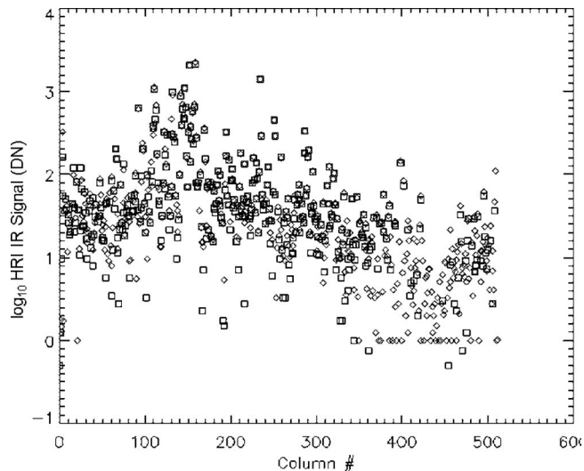
FIG. 90. Application of IR flats to a TV4 HRI-IR Ar-lamp image. Signal from several selected rows is plotted. Squares, original data. Diamonds, data after flat-field division. Little to no improvement in the scatter of the data results from application of the TV4 flat.
