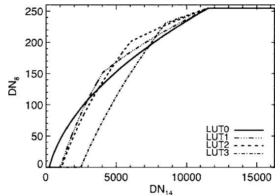
FIG. 13. HRI IR FPA encounter LUTs for converting 14 bit DN 14 to 8 bit DN 8 s.
