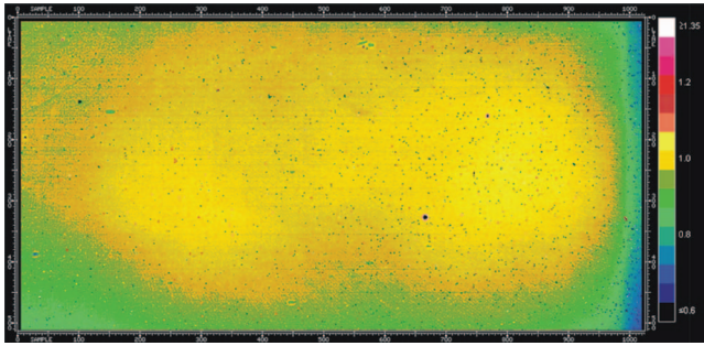
FIG. 92. (Color) Inflight IR spectrometer dark flat field produced using the thermal emission of the optical bench as the illumination source; brightnesses are normalized to the mean value. There is significant spatial structure in the derived flat compared to the TV4 and lunar measurements.
