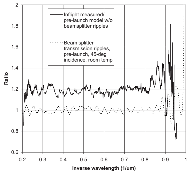
FIG. 84. Residual ratio between the component-level IR spectrometer calibration curve (excluding beamsplitter ripples) and inflight measured curve.
