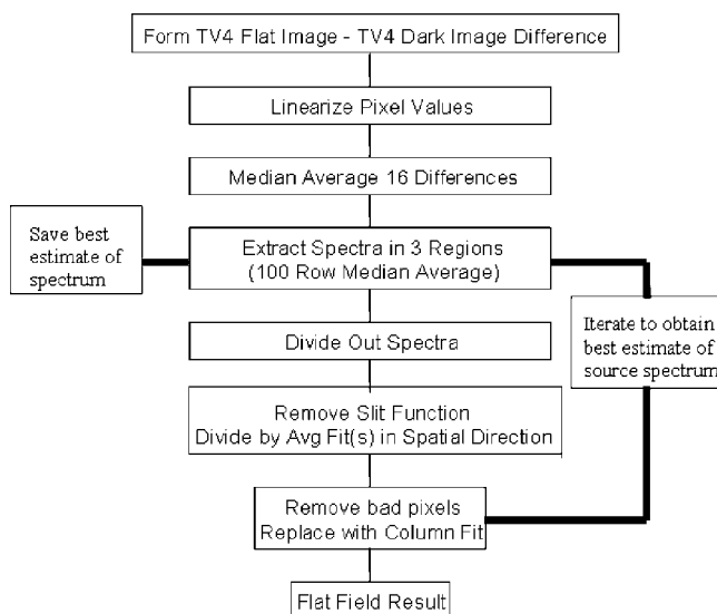
FIG. 87. Flow chart defining the algorithm for deriving the IR spectrometer flat field from images of a spatially uniform source radiance.
