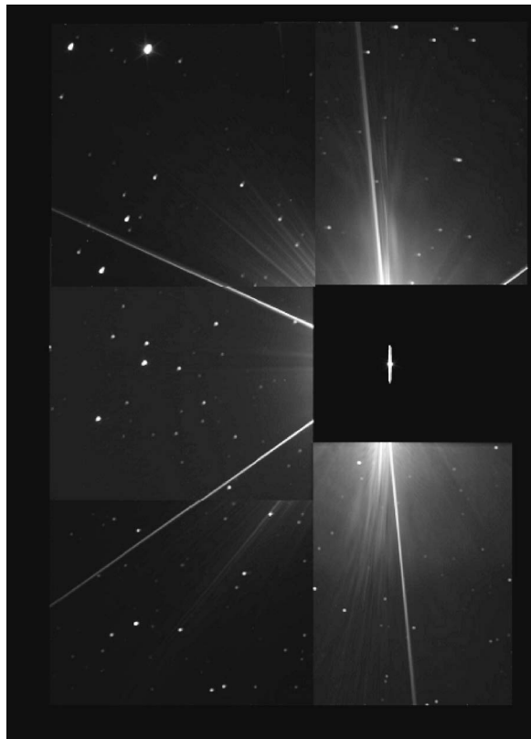
FIG. 42. The stray light pattern for HRI. Canopus is shown scaled as a reference. There are five images surrounding the boresight image. Each image has an exposure time of 800 s. The Canopus image saturates with an exposure time of about 20 ms. The secondary mounting structure (the spider) is the major contributor to the observed stray light.
