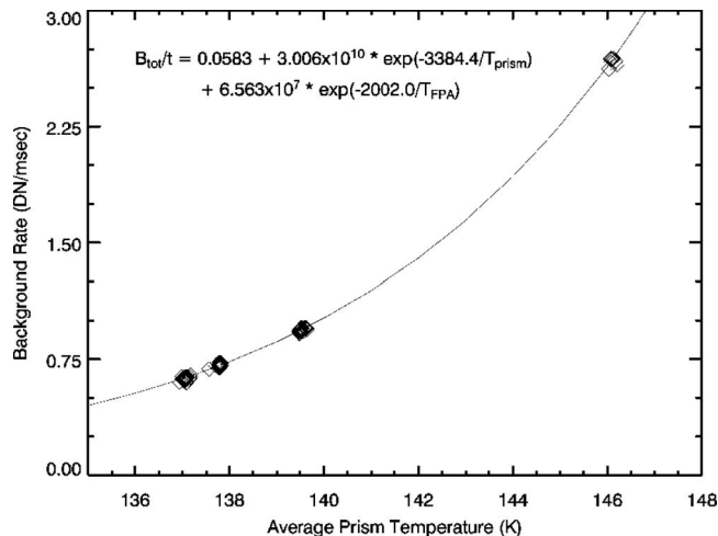
FIG. 72. IR spectrometer background rate as a function of the prism temperature for the in-flight data. Symbols indicate the measured values of the total signal, while the line indicates the computed values for the best fitting modeled contribution from the instrument glow.
