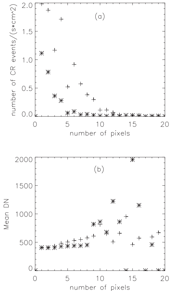
FIG. 52. The number of cosmic ray events per s/cm^2 (top) and mean values of DN (bottom) vs the number of pixels affected by an event at a peak of solar activity (crosses) and for out-of peak activity (stars) on dark MRI images with 9 \leq t \leq 30 s.
