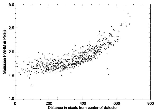
FIG. 18. The PSF FWHM of the ITS star images after bakeout for 710 stars with peak SNR greater than 100 as a function of distance in pixels from the center of the detector.
