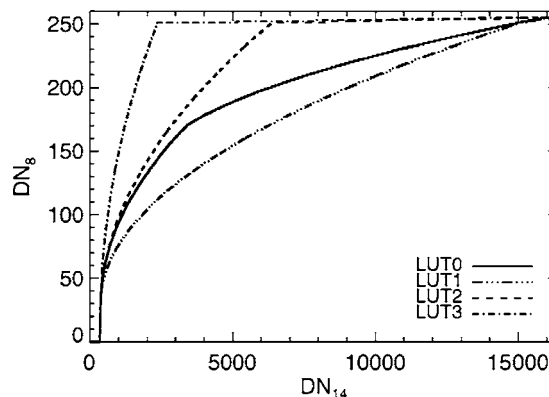
FIG. 10. HRI CCD encounter LUTs for converting 14 bit DNs to 8 bit DNs.
