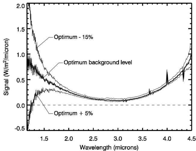
FIG. 77. Example comet spectrum showing the effects of improper IR spectrometer background removal. The heavy line shows the result for the “optimum” background level found as described in the text. The upper thin line shows the result for a 15% decrease in the background level, and the lower thin line shows the result for a 5% increase. Around 3\ \mu\text{m} the effect is \sim 25\% , while at the shortest wavelengths, it overwhelms the signal.
