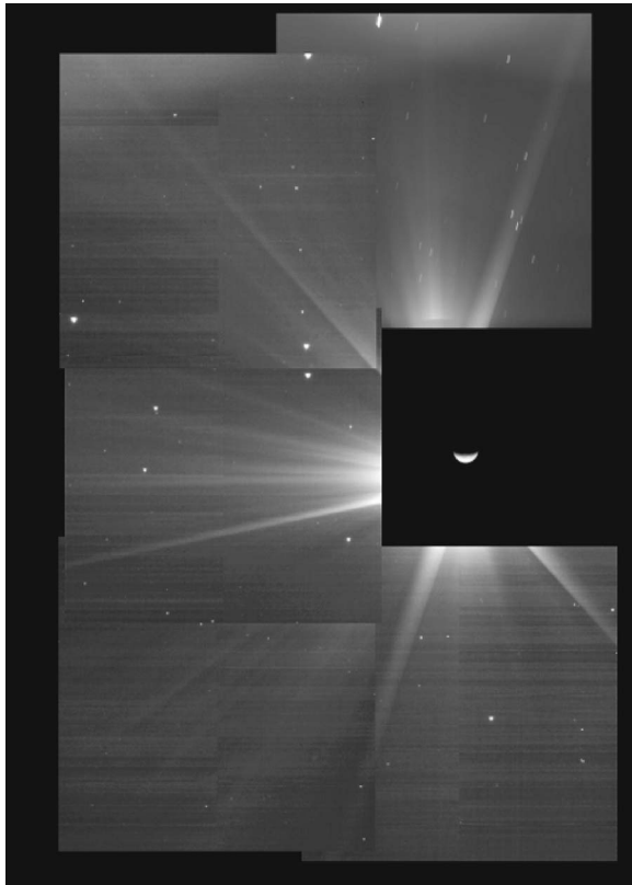
FIG. 45. The stray light for MRI. The moon is shown scaled as reference. There are five images surrounding the boresight image. Each image has an exposure time of 1000 s. The moon saturates with about 15 ms exposure time. The MRI telescope is similar to the HRI, so similar stray light patterns can be seen.
