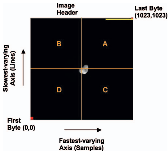
FIG. 8. (Color) A full-frame, MRI image taken at nearly the same time as the HRI vis image in Fig. 7. Displayed with the FITS convention, a true sky image is reproduced (ecliptic north is to the right). The first and last bytes are those read from the FITS file and are not connected with the order of detector readout. Quadrants A–D noted throughout this paper are labeled in the image.
