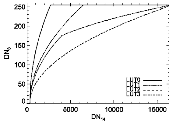
FIG. 103. MRI data compression LUT loaded at launch.
