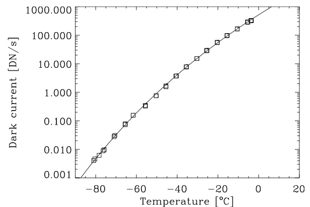
FIG. 24. Dark current as a function of CCD temperature for quadrant C of the HRI instrument. The model is the solid line and the data are the squares.
