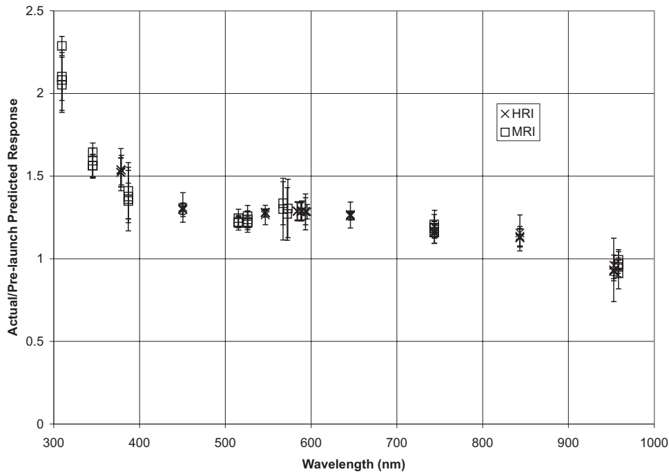
FIG. 29. Ratios of actual inflight stellar response rates to those predicted using the prelaunch camera models.
