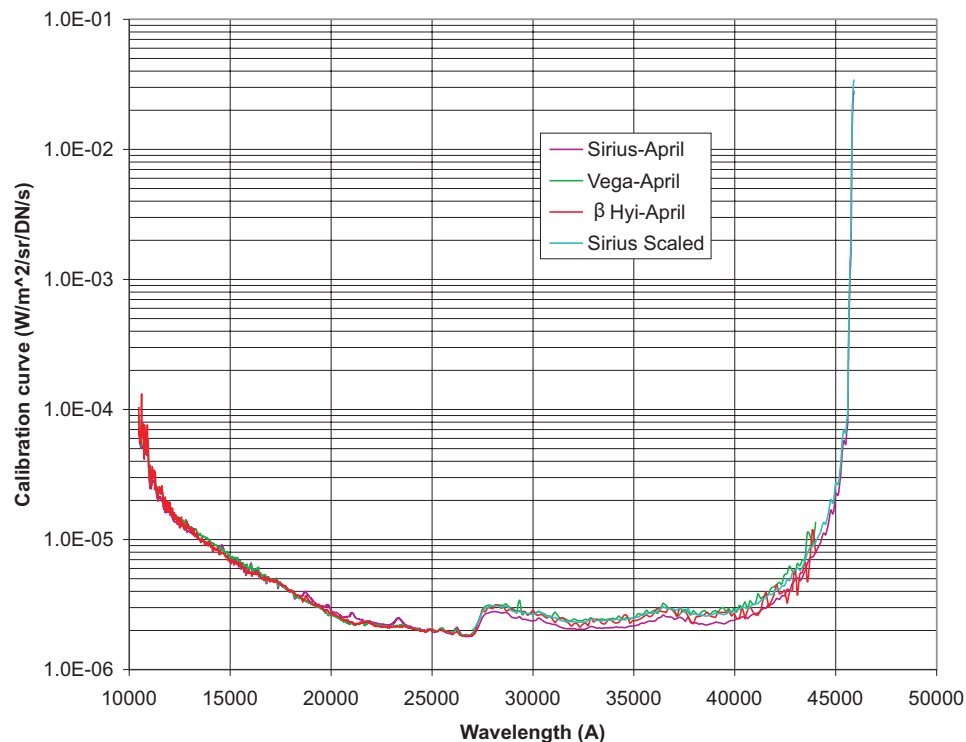
FIG. 81. (Color) IR spectrometer in-flight calibration curves; binned behind antisaturation filter on the top; unbinned outside antisaturation filter on the bottom.
