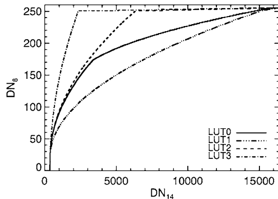
FIG. 11. MRI CCD encounter LUTs for converting 14 bit DN 14 to 8 bit DN 8 s.
