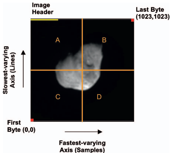
FIG. 7. (Color) A full-frame, HRI vis image taken shortly before impact, displayed with the FITS convention. This orientation reproduces a true sky image (ecliptic north is to the right). The first and last bytes are those read from the FITS file and are not connected with the order of detector readout. Quadrants A–D noted throughout this paper are labeled in the image.
