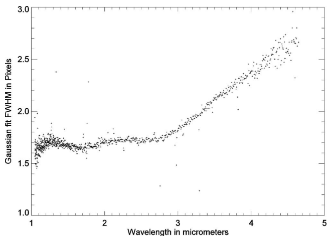
FIG. 65. The IR spectrometer spatial resolution (FWHM of the Gaussian fit in physical pixels) as a function of wavelength for the 10 May 2005 observation of calibration star Beta Hyl. Note that the spatial resolution is dominated by the defocused PSF of the HRI telescope for wavelengths shorter than about 2.8 \mu\text{m} and by the diffraction limit of the telescope for wavelengths longer than about 2.8 \mu\text{m} . One physical pixel is about 8.5 \mu\text{rad} .
