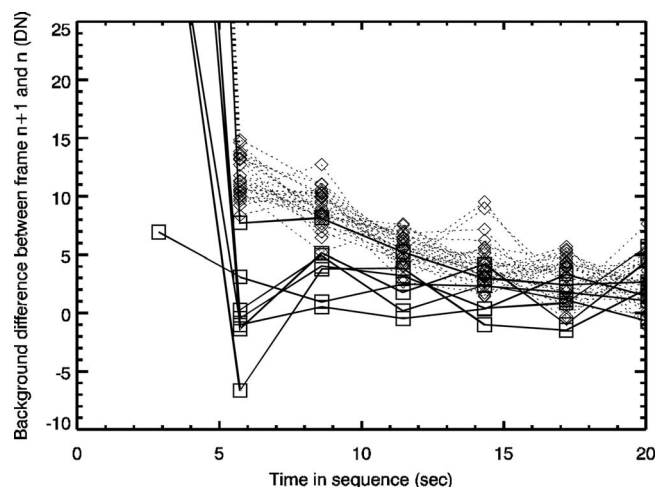
FIG. 76. Falloff in the IR spectrometer background level after the first frame in mode 1. The dotted lines and diamonds show the falloff of the background when the first-frame overshoot reached the plateau, while the solid lines and squares depict the sequences in which the first frame did not reach the plateau level.
