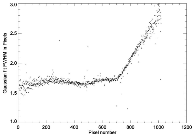
FIG. 64. The IR spectrometer spatial resolution (FWHM of the Gaussian fit) as a function of pixel (column) number for the 10 May 2005 observation of calibration star Beta Hyl. Note that the spatial resolution is approximately constant at a value of 1.6–1.7 pixels FWHM for pixels 6 through about 700 and then rises approximately linearly to nearly 3.0 pixels for pixel numbers around 1000 due to optics diffraction.
