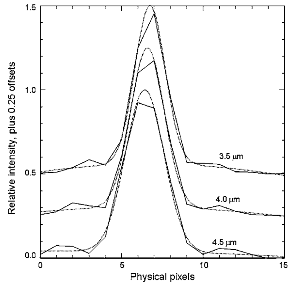
FIG. 66. Along-slit traces of a star image in the IR spectrometer for 3.5, 4.0, and 4.5 \mu\text{m} (top to bottom). Also plotted are Gaussian fits; each data set is normalized by the maximum value of the Gaussian fit and then respectively displaced by 0.5, 0.25, or 0.0 intensity units upwards. The data points are joined by lines, and the Gaussian fit values are dotted.
