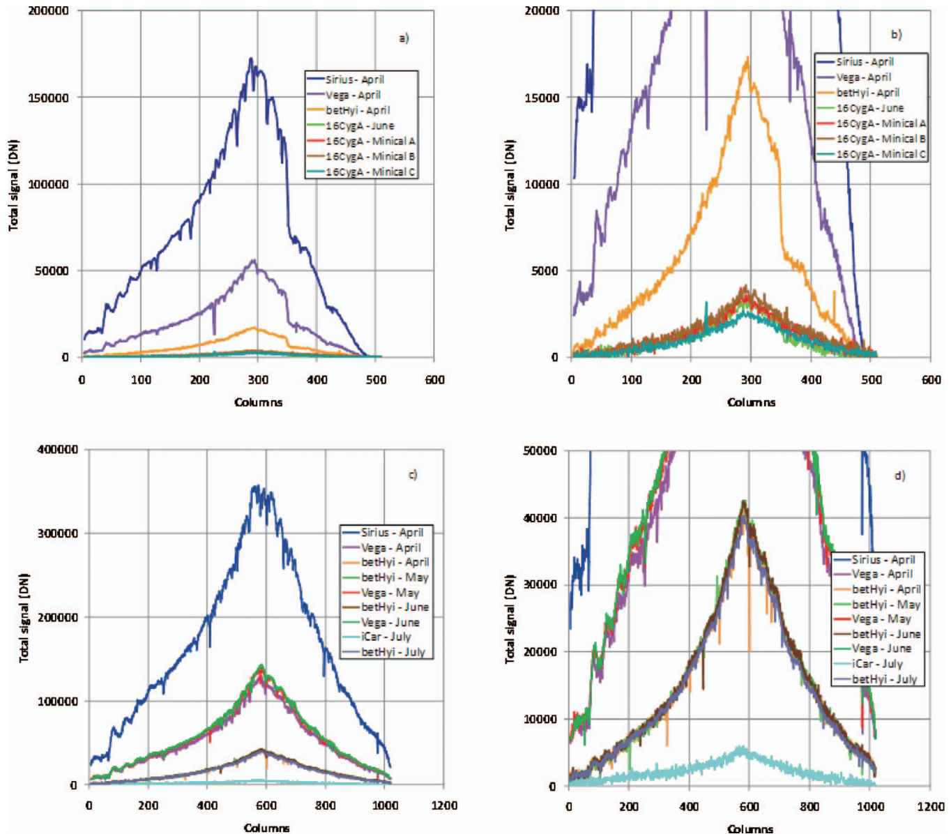
FIG. 80. (Color) IR spectrometer total response during inflight star calibrations: (a) binned mode, behind antisaturation filter except for minicals; (b) binned mode with expanded scale; (c) unbinned mode, all outside antisaturation filter; (d) unbinned with expanded scale.
