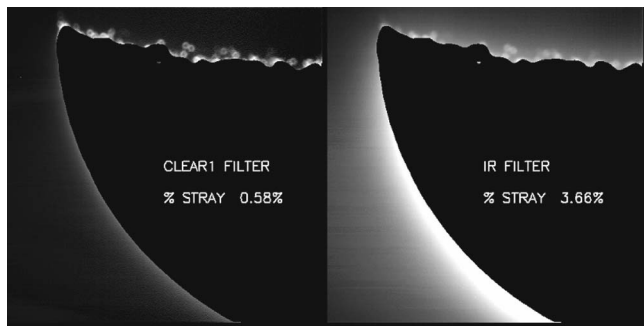
FIG. 48. HRI vis in-field scattered light shows the comparison between the clear filter and the IR filter. Total stray light is expressed as a fraction of the total signal within the masked area. Each image is 512 \times 512 pixels.
