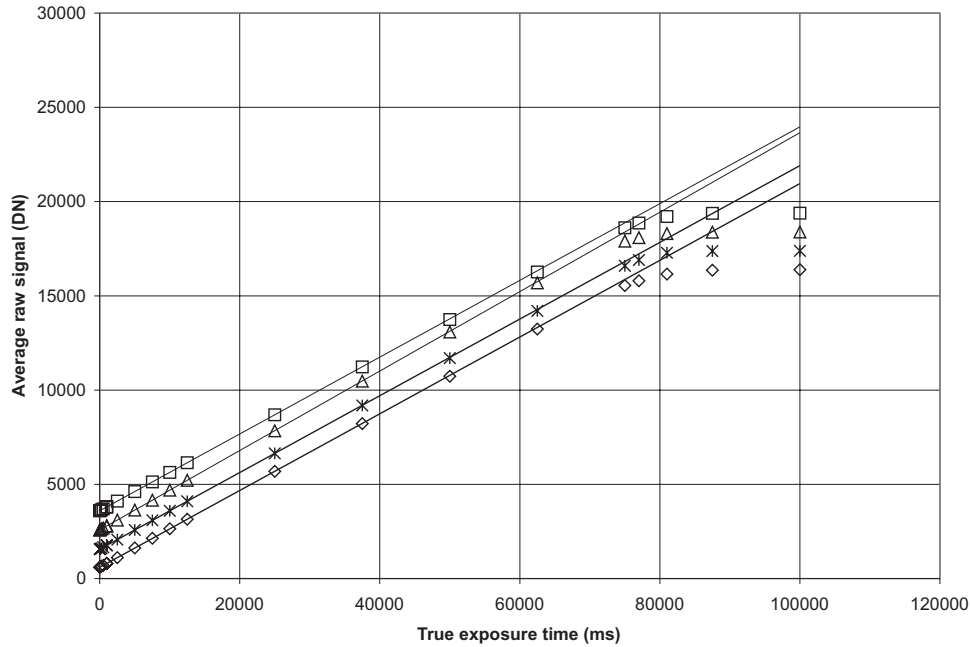
FIG. 21. HRI vis response linearity. Results for the various quadrants are offset by 1000 DN for visibility.
