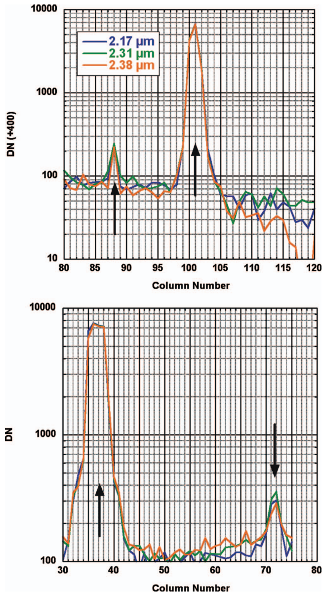
FIG. 99. (Color) Vertical profiles across the IR spectrometer Canopus scans. Top: Scan in the +y direction showing a ghost image at 13 frames ( 325 \mu\text{rad} ) after the star image. Bottom: scan in the -y direction showing a ghost image at 36 frames ( 360 \mu\text{rad} ) after the star image. As described in the text, when corrected for differences in scan rates, the position and magnitude of the ghost images are very similar.
