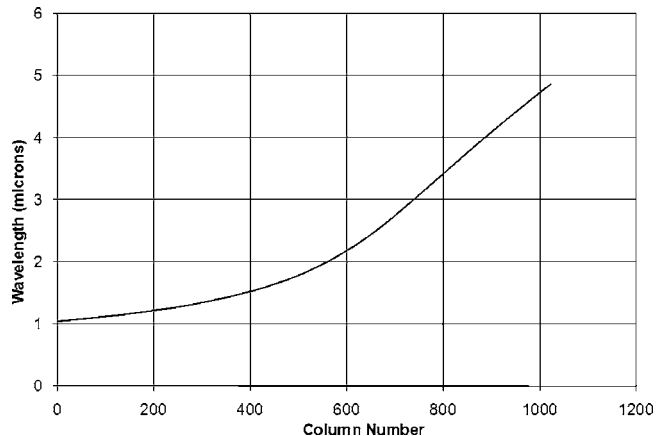
FIG. 78. Wavelength vs unbinned column number for the IR spectrometer for a bench temperature of 140 K.
