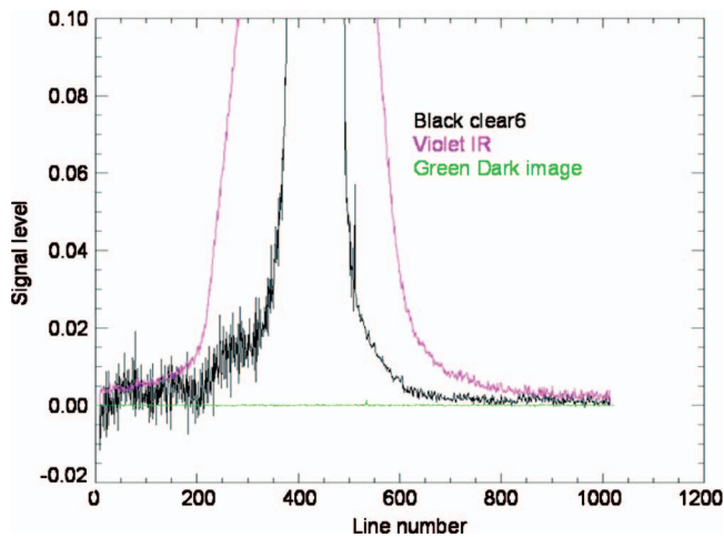
FIG. 50. (Color) MRI in-field scattered light response down column 650. Signal level is in arbitrary units with all filters normalized to the same signal amplitude.
