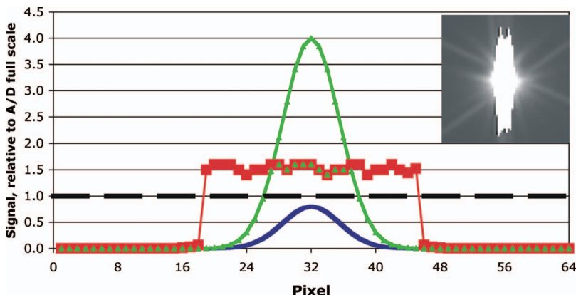
FIG. 51. (Color) CCD saturation and charge conservation. The plot shows an idealized cross section of signal of an unsaturated star (blue line without symbols) and a saturated star (green line with triangles) in the case where the physical limitation of the CCD full well is above the range of the ADC. The signal level is shown relative to the maximum value digitized by the ADC. The resulting signal level in the CCD is also shown (red line with squares). Any signal above the dashed line is digitized as 16 383 counts. The figure in the upper right of the plot is a HRI image of Canopus saturated about 10\times , showing the charge bleeding up and down columns.
