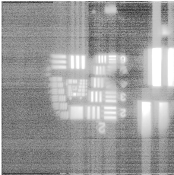
FIG. 25. 100 ms exposure, dark subtracted, Gaussian stretched image showing frame transfer smear.
