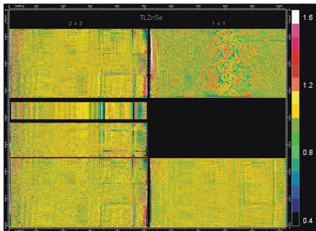
FIG. 89. (Color) Flat-field IR spectrometer images obtained during TV4 with the W lamp through the ZnSe window; brightnesses are normalized to the mean value. From top to bottom on the left are modes 5, 3, 2, and 1 flats, and on the right are modes 6 and 4. Wavelength varies from 1 to 5 \mu\text{m} from left to right in each image. Residual structures, some likely due to the illumination pattern of the W lamp reflecting off a rough gold surface, are apparent in both the dispersion (horizontal) and spatial (vertical) directions.
