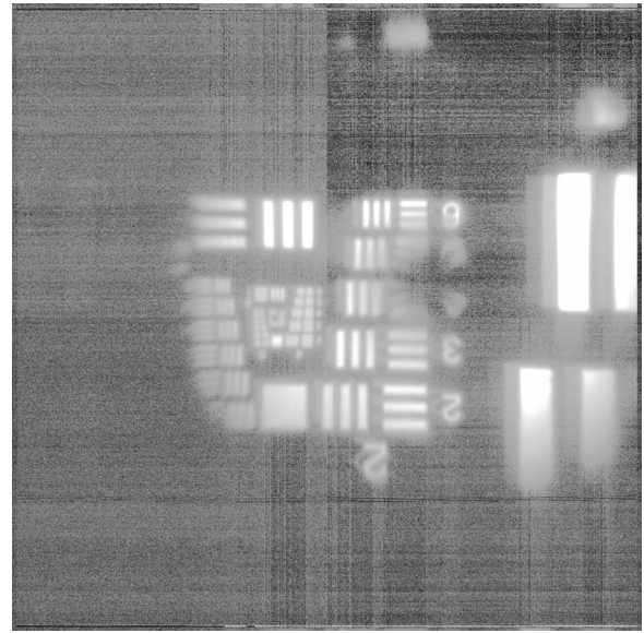
FIG. 26. Version of Fig. 25 corrected for frame transfer smear using parallel overlocked pixel value.
