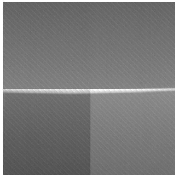
FIG. 39. CCD room-temperature dark current pattern. The center 256 \times 256 pixels of a room-temperature HRI image are shown.
