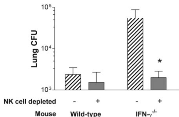
FIG. 3. Mycoplasma CFU found in lungs of anti-asialo GM-1 antibody-treated and untreated wild-type and IFN-\gamma^{-/-} mice. Wild-type and IFN-\gamma^{-/-} mice were depleted of NK-like cells on day -1 by use of treatment with anti-asialo GM1 antibody. Three days postinfection, the numbers of mycoplasma CFU in lungs were determined. Vertical bars and error bars represent means \pm SE ( n = 8 ). "*" denotes a statistical difference ( P \leq 0.05 ) from strain control results.
