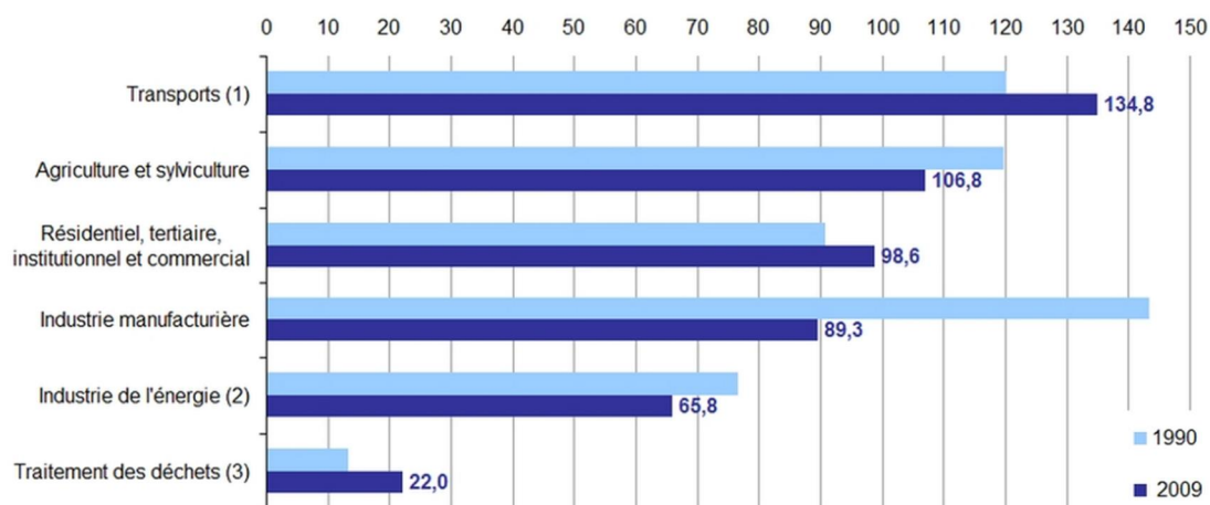
Figure: Evolution of transport CO 2 emissions in mTCO 2 eq between 1990 and 2009 73
