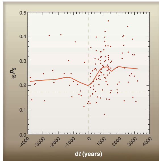
Fig. 1. The proportion of 5- to 19-year-old skeletons (to all skeletons 5 or more years old) (vertical axis: {}_{15}P_5 ) in 133 cemeteries across the Northern Hemisphere during the transition from foraging to farming (horizontal axis: dt ). The horizontal axis dt represents the time that elapsed between the advent of farming at that particular location, aligned at dt = 0 [from (25)]. (Below) The population explosion of the Neolithic Demographic Transition, detectable in cemeteries, was unprecedented in the history of Homo sapiens . Neolithic gallery grave of La Chaussée Tirancourt, France (~4500 years before the present).
