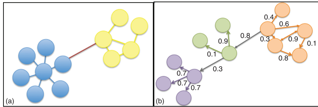
Figure 1 Example networks: (a) unweighted and undirected; (b) weighted and directed.
