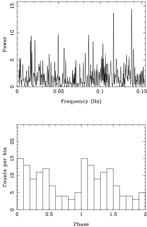
Figure 3. The power spectrum and folded light curve resulting from a Z^2 statistical search for periodicity from AX J144701–5919 as output by ChIcAGO MAP. Top: The power spectrum (power vs. frequency (Hz)) of AX J144701–5919. The power spectrum peaks at a value of Z_1^2 = 14.4 at a frequency of 0.1378 Hz. The probability of this power being random noise is 0.16. It is therefore unlikely to be a real signal. Bottom: The folded light curve (counts per bin vs phase) that has been folded at 0.1378 Hz.
