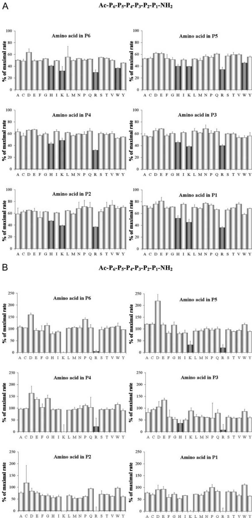
Fig. 1. Screening of L-hexapeptides PS-SPCL for in vitro inhibition of PC5/6 (A) and PC7 (B) activity. Each mixture is defined by a specified L-amino acid for one of the six positions of the hexapeptide sequence. The remaining five positions are composed of a mixture of 19 L-amino acids (all except cysteine). For example, at the panel “Amino acid in P1,” only the P 1 position is defined and the other positions are random: Ac-X-X-X-X-P 1 -NH 2 . Inhibition or activation of enzymatic activity in the presence of peptide mixtures is given as a percentage of maximum rate relative to that of controls. The most inhibitory amino acids for each position are shaded in black.
