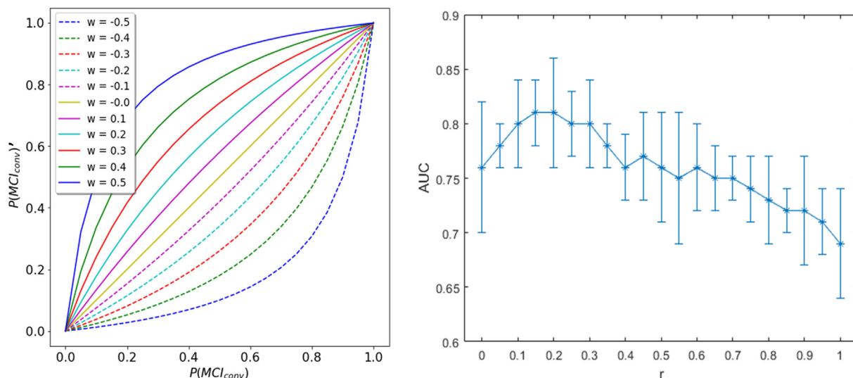
Fig. 2. Curves for P(MCI_{conv})' vs. P(MCI_{conv}) under different settings of w^i ( r = 0.8 ).
