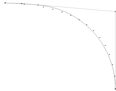
Fig. 4. Second example: (a) biarc with r = 1 ; (b) biarc with Sabin's constraint; (c) biarc with \hat{r} = 4.692 .
