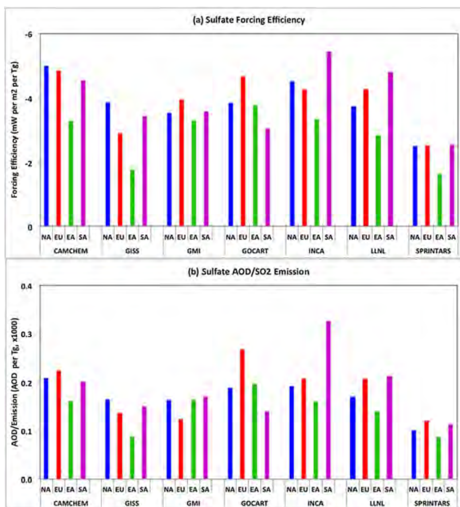
Figure 7. Global annual mean (a) forcing efficiency ( \text{mW m}^{-2} per Tg) and (b) AOD/emission ( \text{AOD per Tg} \times 1000 ) attributed to 20% anthropogenic emissions in individual source regions (denoted as NA, EU, EA, and SA) as simulated by seven HTAP models.
