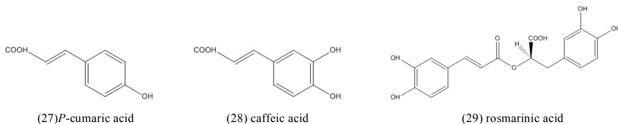
Fig. (5). Structure of Phenylpropanoids.
