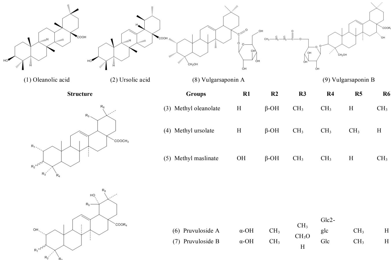
Fig. (1). Structures of triterpenes.
