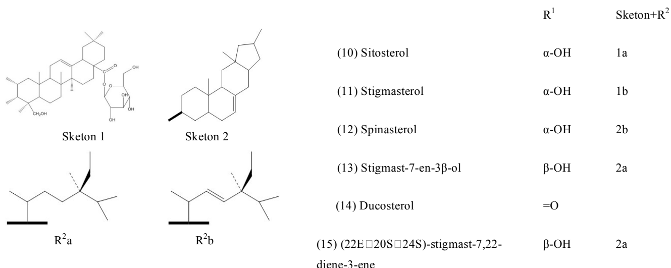
Fig. (2). Structures of steroids and derivatives.
