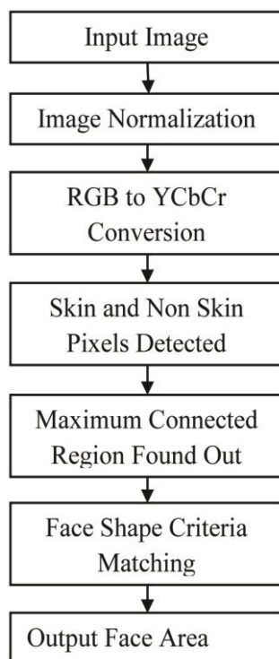
Figure 3. Sample of Skin Color Detection Algorithm [36]
