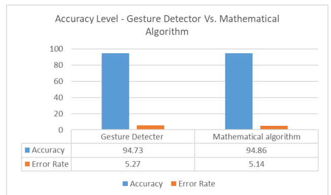
Figure 20 - Accuracy Level of Gesture Detector over Mathematical Algorithm
