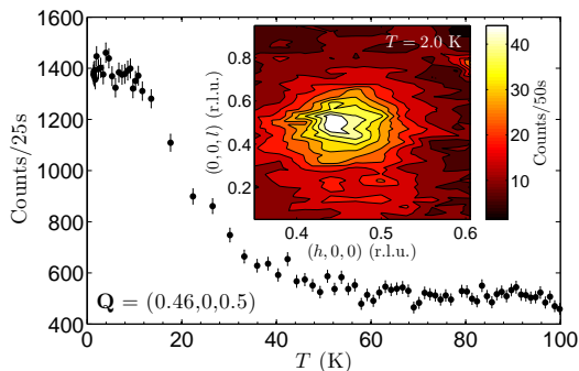
FIG. 3: (Color online) Neutron diffraction from \text{Fe}_{1.03}\text{Se}_{0.25}\text{Te}_{0.75} . The contour plot maps the spin-flip scattering of polarized neutrons in the (h, 0, l) plane, and reveals an incommensurate magnetic peak at (0.46, 0, 0.5) . The main plot shows the temperature dependence of the intensity at (0.46, 0, 0.5) measured with unpolarized neutrons.
