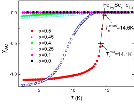
FIG. 1: (Color online) Temperature dependence of the AC volume susceptibility \chi_{AC} of \text{Fe}_{1+y}\text{Se}_x\text{Te}_{1-x} . The onset T_c^{\text{onset}} and mid-point T_c^{\text{mid}} of the superconducting transition are determined from the intersection of straight lines fit to the data above and below the transition, and the point corresponding to \chi_{AC} = -0.5 , respectively.
