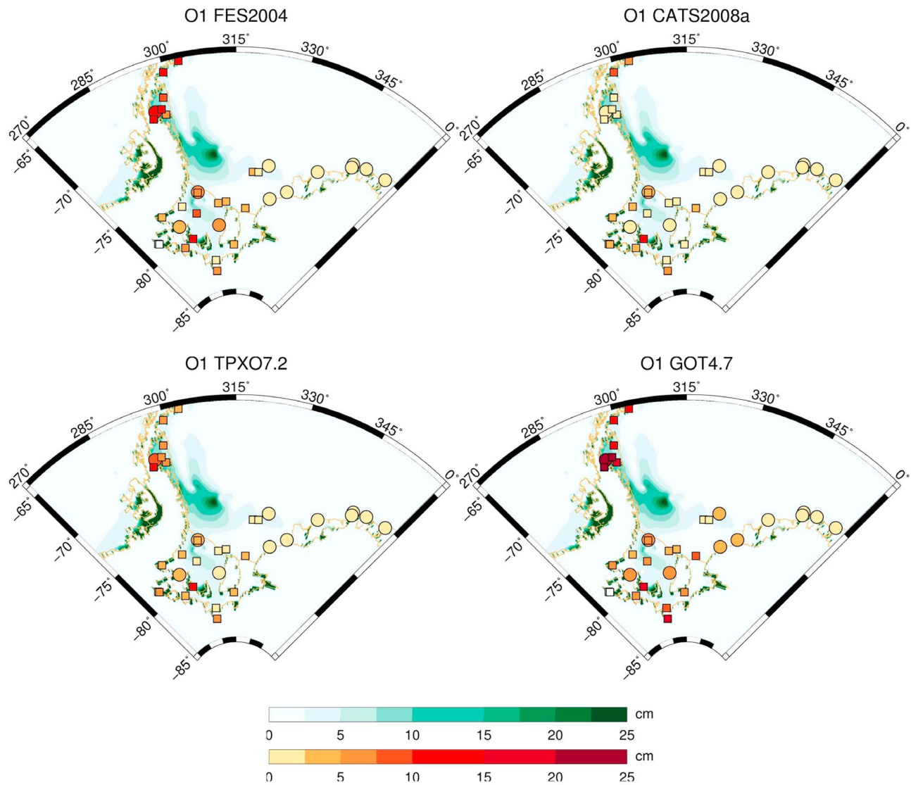
Figure 4. Same as for Figure 2 but for O1.
