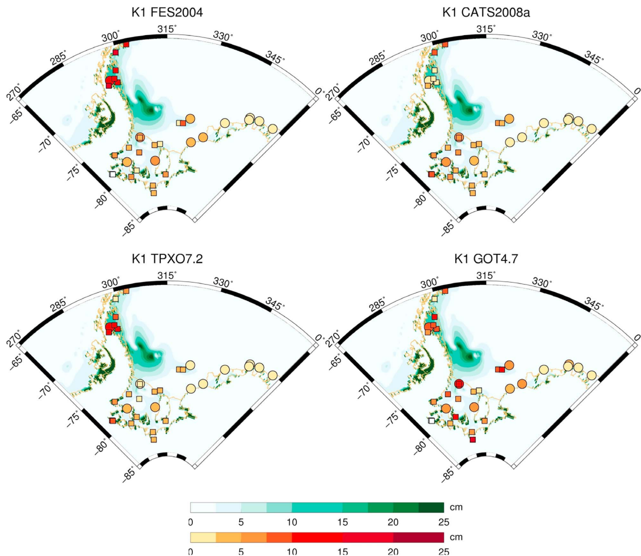
Figure 5. Same as for Figure 2 but for K1.
