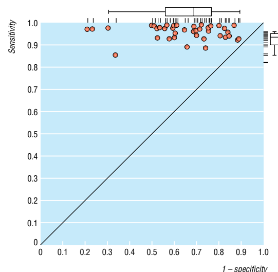
Fig 2 Receiver operating characteristics plot of all included studies (39 2×2 tables)
