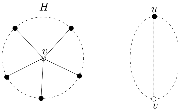
Figure 7.1: An odd wheel and a 3-odd-path configuration
