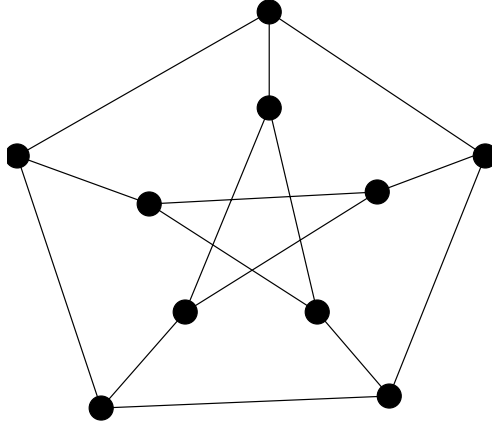
Figure 1.1: The Petersen graph.
