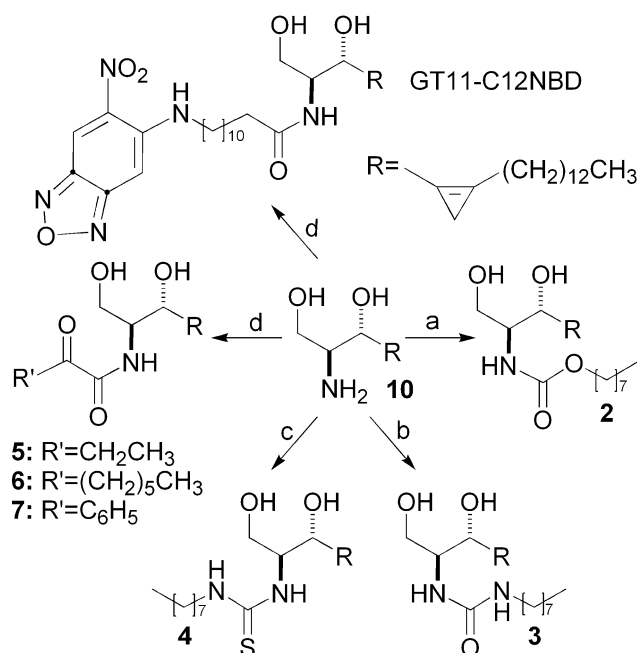
Scheme 2 Synthesis of 2–7 and GT11-C12NBD. a, \text{CH}_3(\text{CH}_2)_7\text{CO}_2\text{Cl} in methylene chloride–triethylamine; b, \text{CH}_3(\text{CH}_2)_3\text{NCO} in diethyl ether–acetonitrile; c, \text{CH}_3(\text{CH}_2)_5\text{NCS} in diethyl ether–acetonitrile; d, treatment with the appropriate acid in the presence of EDC–HOBT in either methylene chloride or diethyl ether–acetonitrile. Acids are \text{NBD}(\text{CH}_2)_{11}\text{COOH} (GT11-C12NBD); \text{CH}_3\text{CH}_2\text{COCOCH}_3 ( 5 ); \text{CH}_3(\text{CH}_2)_5\text{COCOCH}_3 ( 6 ) and \text{C}_6\text{H}_5\text{COCOCH}_3 ( 7 ).
