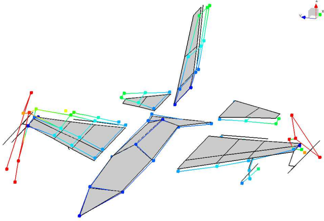
(c) Second mode at 6.18 Hz: antisymmetric missile rotation.
