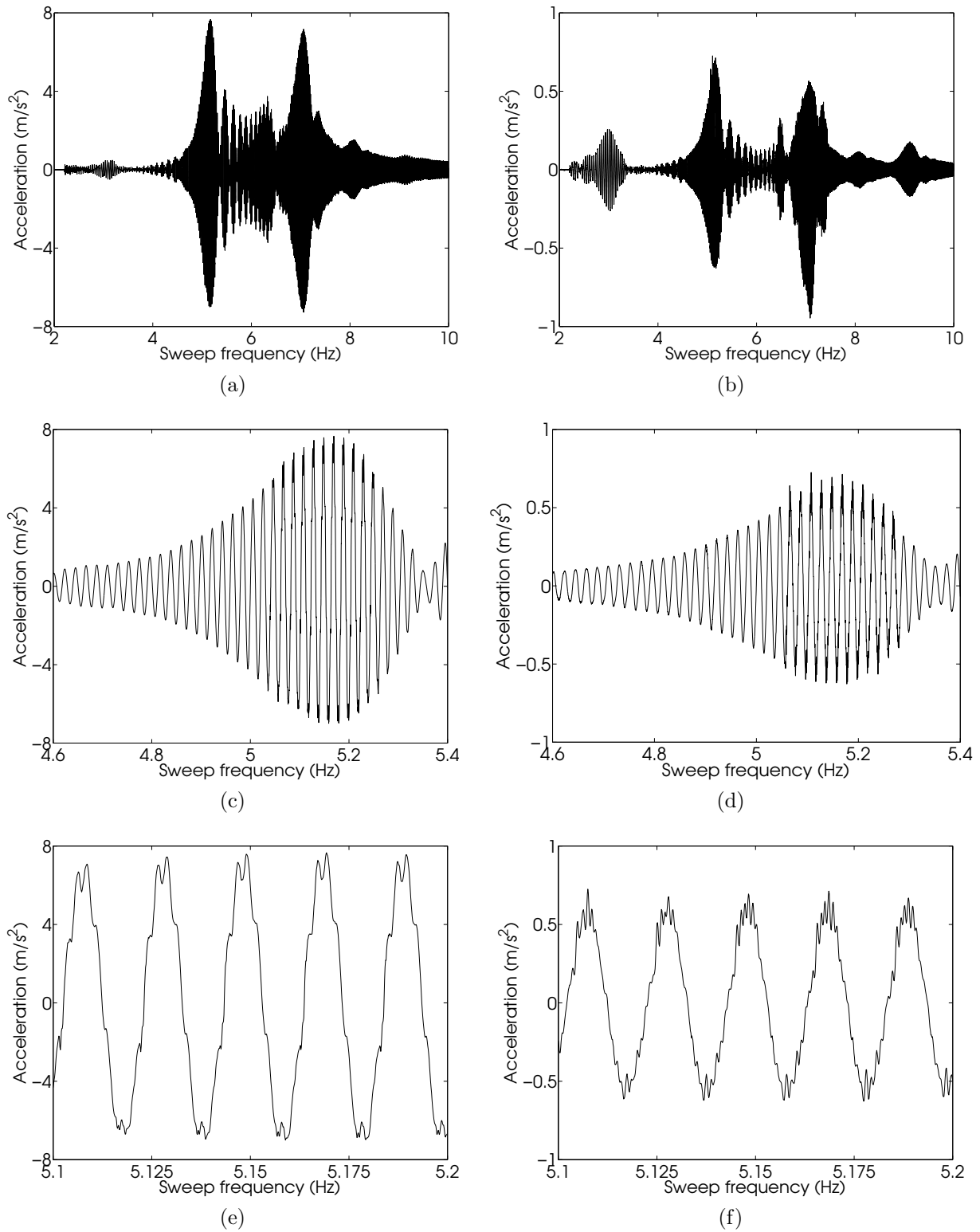
Figure 5: Accelerations measured on the dummy missile mounted to the right wing (left column) and on the dummy bomb (right column) for 3 sweep frequency intervals. (a – b) 2 – 10 Hz; (c – d) 4.6 – 5.4 Hz; (e – f) 5.1 – 5.2 Hz.
