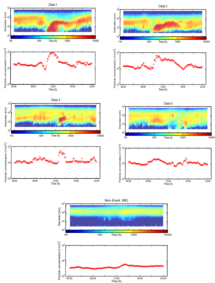
Fig. 2. Examples of new particle formation and event classification.
