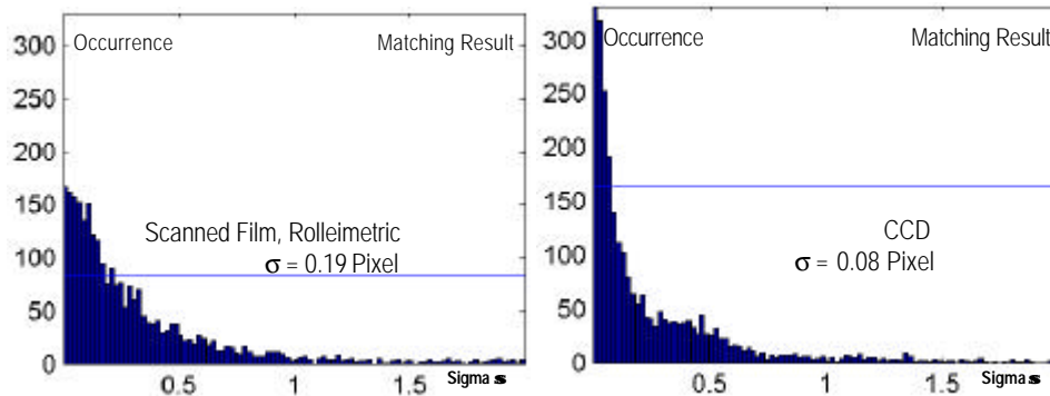
Figure 4: Comparing matches from a pair of scanned film images (at 15µm pixel size) and from a pair of digitally sensed images. The histograms show that the film-based matches have larger errors. The errors are obtained by determining the distance of each match point from the corresponding epipolar ray. The CCD-based matches have a noise level that is 2.4 times smaller than the matches based on scanned film.
