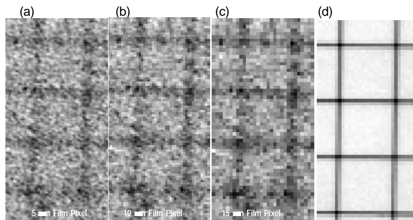
Figure 1: Images of a grid pattern. (a) through (c) were obtained by scanning a film image using pixel sizes of 5µm, 10µm and 15µm. The digital image in (d) has a pixel size of 12µm. It clearly outperforms all of the film scans. Film does not seem to contain sufficient information to compete with a 12µm digital pixel (Perko and Gruber, 2002).
