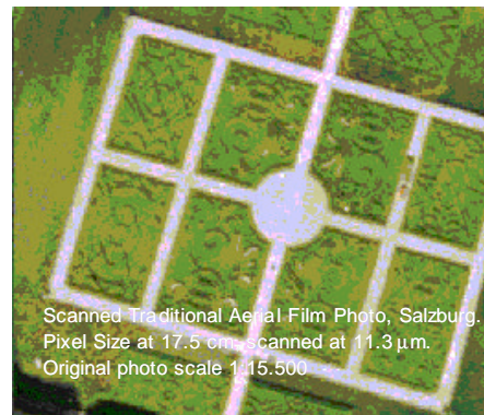
Figure 5: Comparing scanned aerial film with a digital aerial image from UltraCam-D. Both images produce 17.5 cm pixels on the ground. The images were taken one year apart; therefore some changes have occurred on the ground. Important is the fact that the film image was taken after a rain with water on the ground. The digital image was taken during a dry period.
