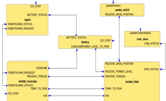
Figure 7: Design of a robotic arm for an orbital mission using TASTE
