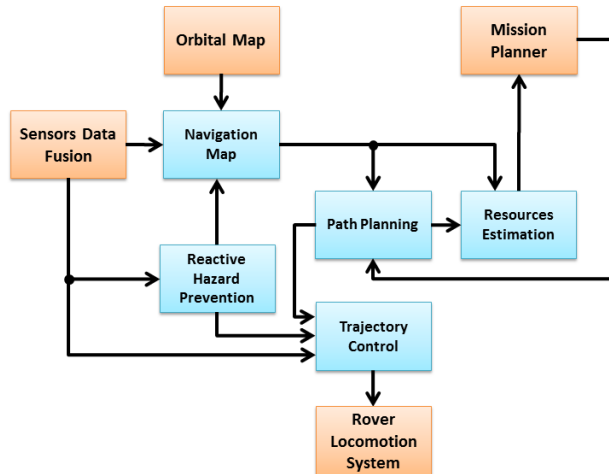
Figure 6: The rover guidance includes (in blue): building of a navigation map, path planning, hazard prevention, trajectory control and resources estimation
