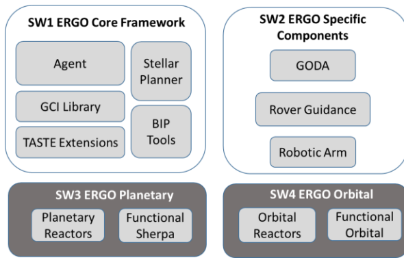
Figure 1: ERGO Framework packages
