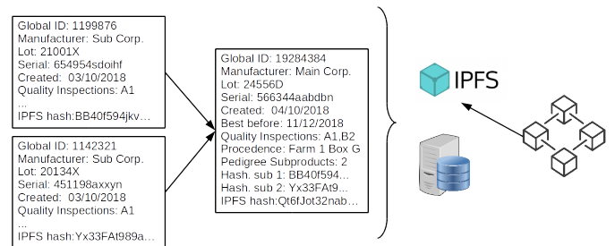
Fig. 3. Overview of the architecture's storage management.
