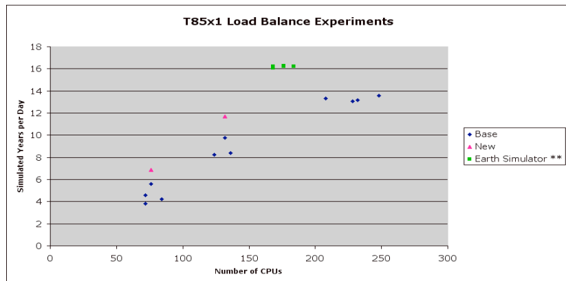
Figure 6: T85x1 Performance Estimates
