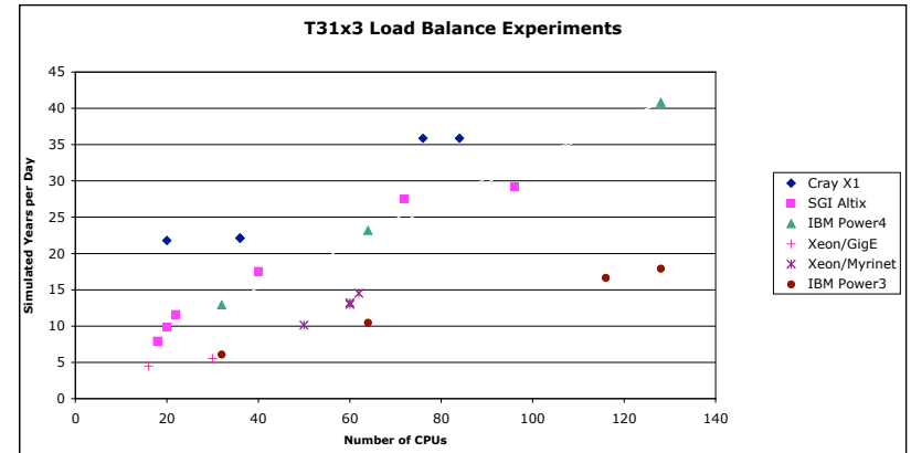
Figure 3: Load Balance Experiments (Performance)
