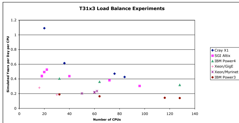
Figure 4: Load Balance Experiments (Efficiency)
