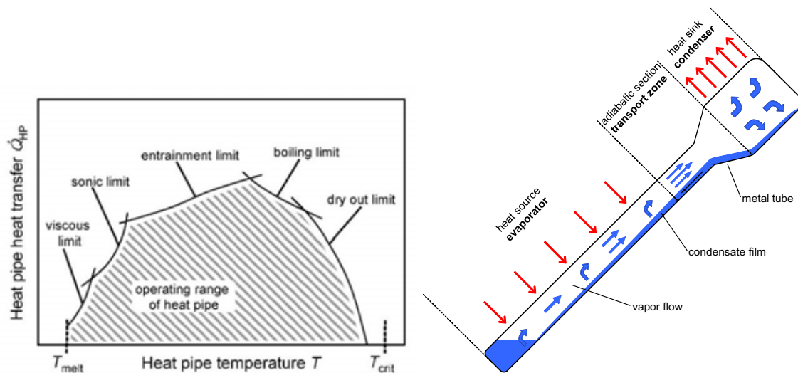
Fig. 1: Reduced operating range of gravitational heat pipes due to melting temperature and critical temperature of the working fluid as well as operation limits (left; Faghri, 1995) and schematic illustration of a gravitational heat pipe for solar collectors (right)
