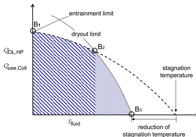
Figure 5: Schematic representation of the design criteria taking into account the required heat transfer rates and the heat transfer limits, depending on the temperature of the solar circuit fluid.
