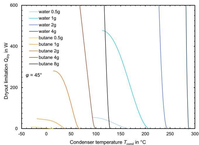
Fig. 3: Calculated dry-out limits of gravitational heat pipes for solar thermal collectors with different types and amounts of working fluids
