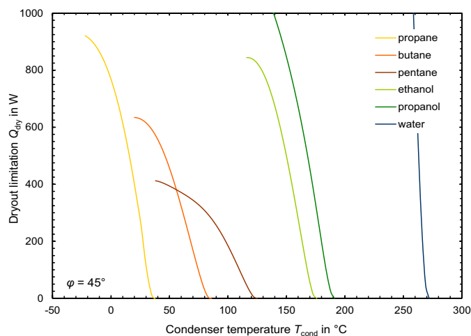
Fig. 2: Calculated dry out limits of gravitational heat pipes for solar thermal collectors filled with different working fluids
