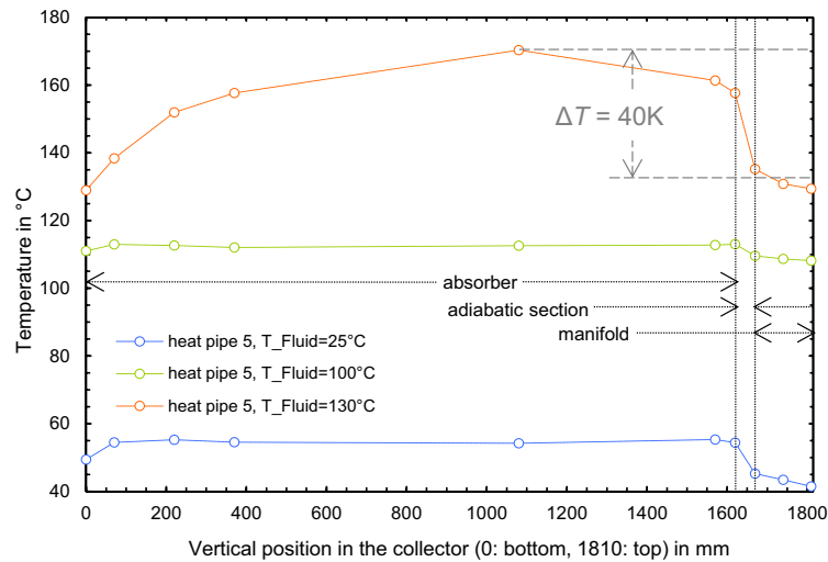
Figure 8: Measurement results of the temperature distribution along a heat pipe at the center of the collector P.1 for the operating point at 25 °C and 100 °C mean fluid temperature, and for the case of stagnation ( T_{\text{fluid}} = 130 °C)
