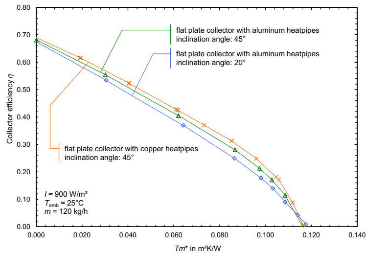
Figure 7: Measured efficiency curves of novel flat-plate collector prototypes with reduced performance at high temperatures due to the use of deactivating heat pipes for different tube materials and inclination angles.
