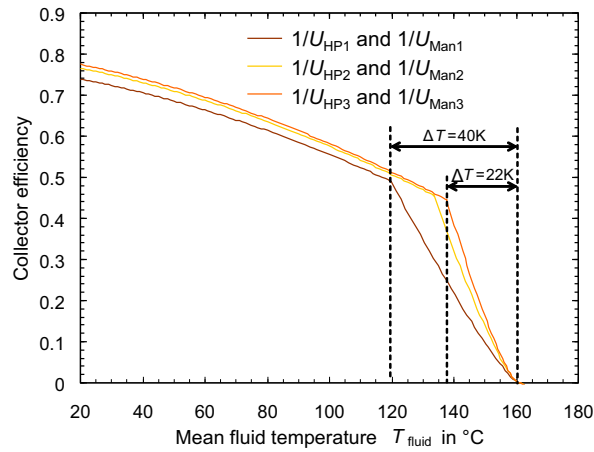
Fig. 4: Calculated influence of the thermal resistances of the heat pipe and the manifold on the collector efficiency and the shut down behaviour of a standard evacuated tube collector with an alkane as working fluid.
