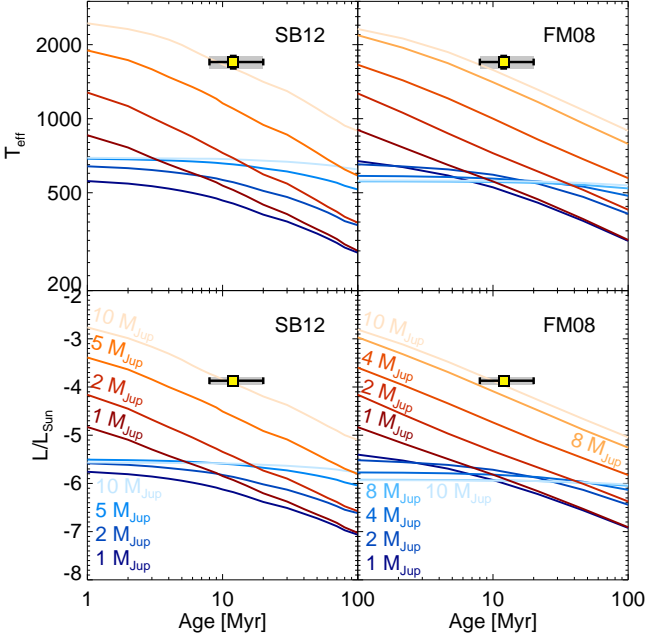
Fig. 10. Luminosity and effective temperatures of \beta Pictoris b compared to those predicted by “cold-start” (blue curves) and “hot-start” (red curves) models of Fortney et al. (2008) –FM08– and Spiegel & Burrows (2012) –SB12– at solar metallicity for different masses and ages.
