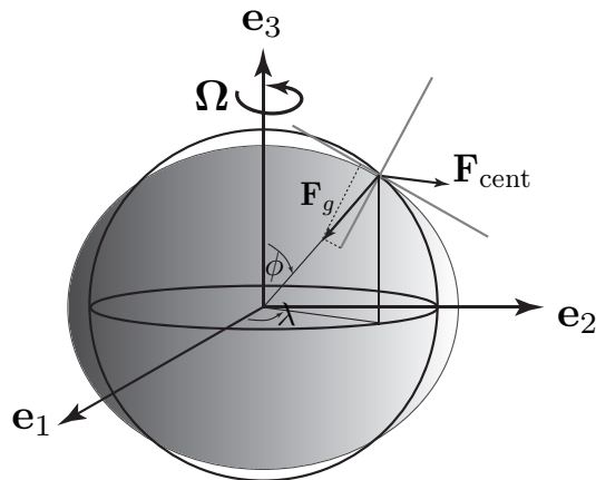
Fig. 1. The earth (oblate spheroid) is modeled as a rotating sphere with an added potential used to emulate the effect of the eccentricity which produces a non-zero horizontal component of gravity.
