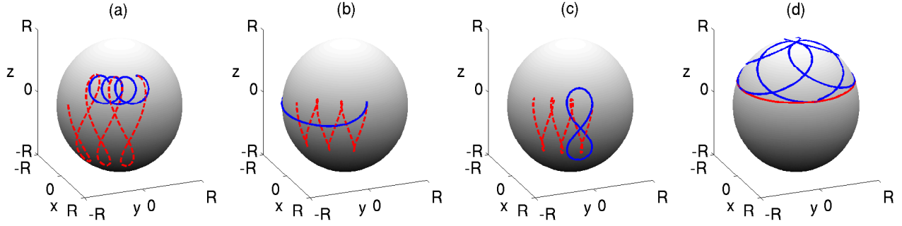
Fig. 2. Free motion of a particle of mass m on a rotating earth and rotating sphere, the solid line is the trajectory on earth, dashed line is on sphere. End time is 3 days for all examples, initial conditions are: (a) (\phi_0, \lambda_0) = (\pi/4, 0) , (\dot{\phi}_0, \dot{\lambda}_0) = (0, 2) ; (b) (\phi_0, \lambda_0) = (3\pi/8, 0) , (\dot{\phi}_0, \dot{\lambda}_0) = (0.92, 0) ; (c) (\phi_0, \lambda_0) = (3\pi/8, 0) , (\dot{\phi}_0, \dot{\lambda}_0) = (1.366, 0) ; (d) (\phi_0, \lambda_0) = (3\pi/8, 0) , (\dot{\phi}_0, \dot{\lambda}_0) = (0, -2\pi) .
