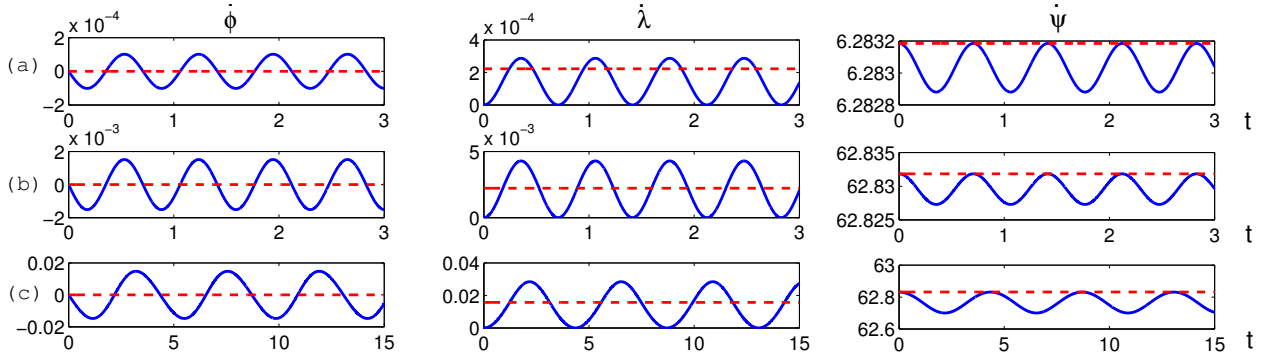
Fig. 3. Free motion of a spinning disc on rotating earth, the solid line is the result of direct numerical integration, dashed line is an approximate solution. We present \dot{\phi} , \dot{\lambda} and \dot{\psi} in three columns respectively. Initial conditions and end times are: (a) (\phi_0, \lambda_0) = (\pi/4, 0) , (\dot{\phi}_0, \dot{\lambda}_0, \dot{\psi}_0) = (0, 0, \Omega) , end time 3 days; (b) (\phi_0, \lambda_0) = (\pi/4, 0) , (\dot{\phi}_0, \dot{\lambda}_0, \dot{\psi}_0) = (0, 0, 10\Omega) , end time 3 days; (c) (\phi_0, \lambda_0) = (\pi/2 - 0.1, 0) , (\dot{\phi}_0, \dot{\lambda}_0, \dot{\psi}_0) = (0, 0, 10\Omega) , end time 15 days.
