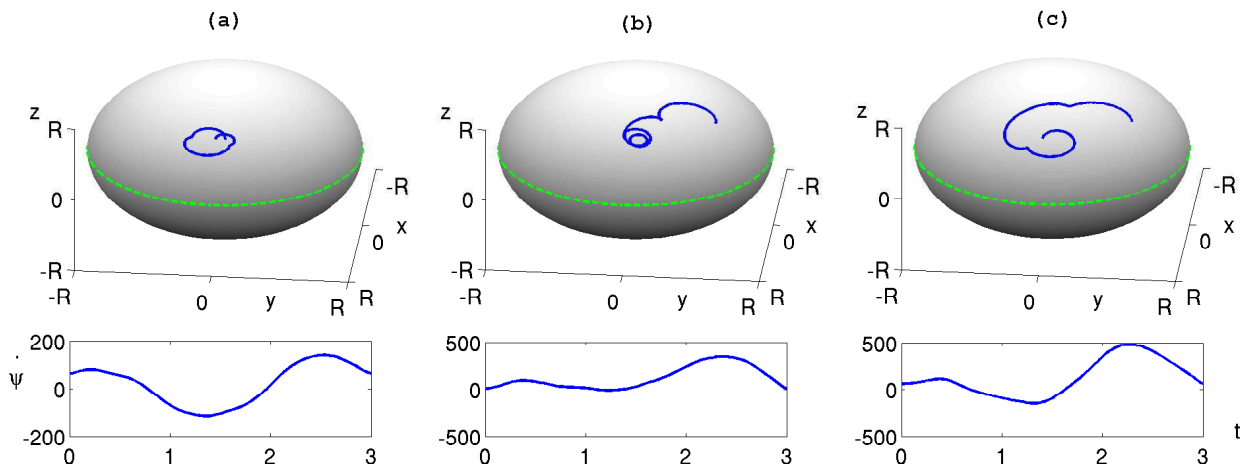
Fig. 5. Optimal control results of the spinning disc on rotating earth. In the first row, we show trajectories in solid line and the equator in dotted line. In the second row, we present the spinning velocities correspondingly. End time is 3 days for all examples. Initial and final conditions are: (a) (\phi_0, \lambda_0) = (\pi/4, 0) , (\dot{\phi}_0, \dot{\lambda}_0, \dot{\psi}_0) = (0, 0, 10\Omega) , (\phi_f, \lambda_f) = (\pi/4, 0.1) , (\dot{\phi}_f, \dot{\lambda}_f, \dot{\psi}_f) = (0, 0, 10\Omega) ; (b) (\phi_0, \lambda_0) = (\pi/4, 0) , (\dot{\phi}_0, \dot{\lambda}_0, \dot{\psi}_0) = (0, 0, \Omega) , (\phi_f, \lambda_f) = (\pi/4, \pi/3) , (\dot{\phi}_f, \dot{\lambda}_f, \dot{\psi}_f) = (0, 0, \Omega) ; (c) (\phi_0, \lambda_0) = (\pi/4, 0) , (\dot{\phi}_0, \dot{\lambda}_0, \dot{\psi}_0) = (0, 0, 10\Omega) , (\phi_f, \lambda_f) = (\pi/4, \pi/3) , (\dot{\phi}_f, \dot{\lambda}_f, \dot{\psi}_f) = (0, 0, 10\Omega) .
