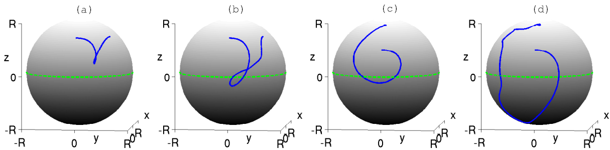
Fig. 4. Optimal control results of particle on rotating earth, the solid line is trajectory under control, and dashed line is equator. Initial and final conditions for case (a) and (b) are: (\phi_0, \lambda_0) = (\pi/4, 0) , (\phi_0, \lambda_0) = (0, 0) , (\phi_f, \lambda_f) = (\pi/4, \pi/3) , (\phi_f, \lambda_f) = (0, 0) , and the end times: (a) t_f = 1 day, (b) t_f = 3 days. Initial and final conditions for case (c) and (d) are: (\phi_0, \lambda_0) = (\pi/3, 0) , (\phi_0, \lambda_0) = (0, 0) , (\phi_f, \lambda_f) = (\pi/8, 0) , (\phi_f, \lambda_f) = (0, 0) , and the end times: (c) t_f = 1 day, (d) t_f = 3 days.
