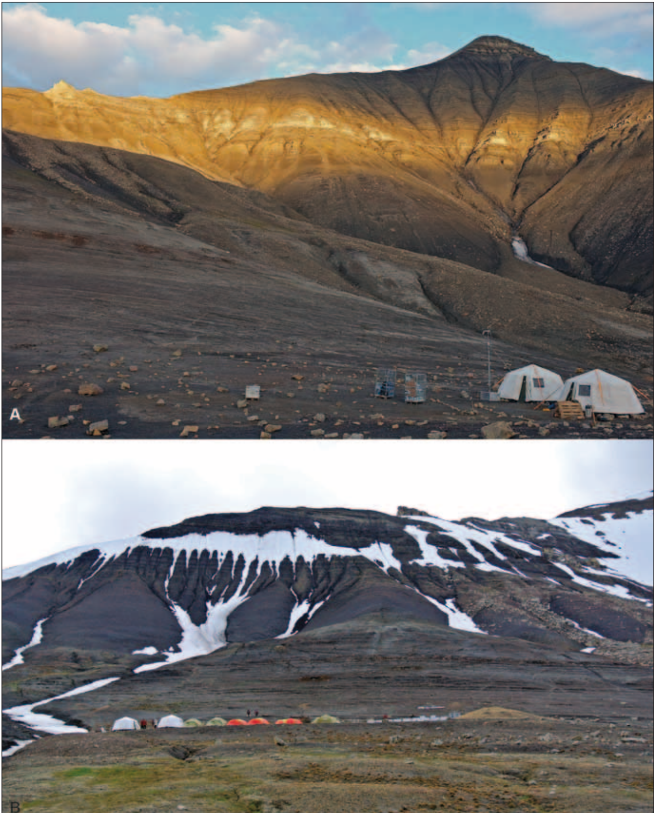
Figure 4. Photo of camp and typical outcrops in A. Janusfjellet. B. Wimanfjellet.
