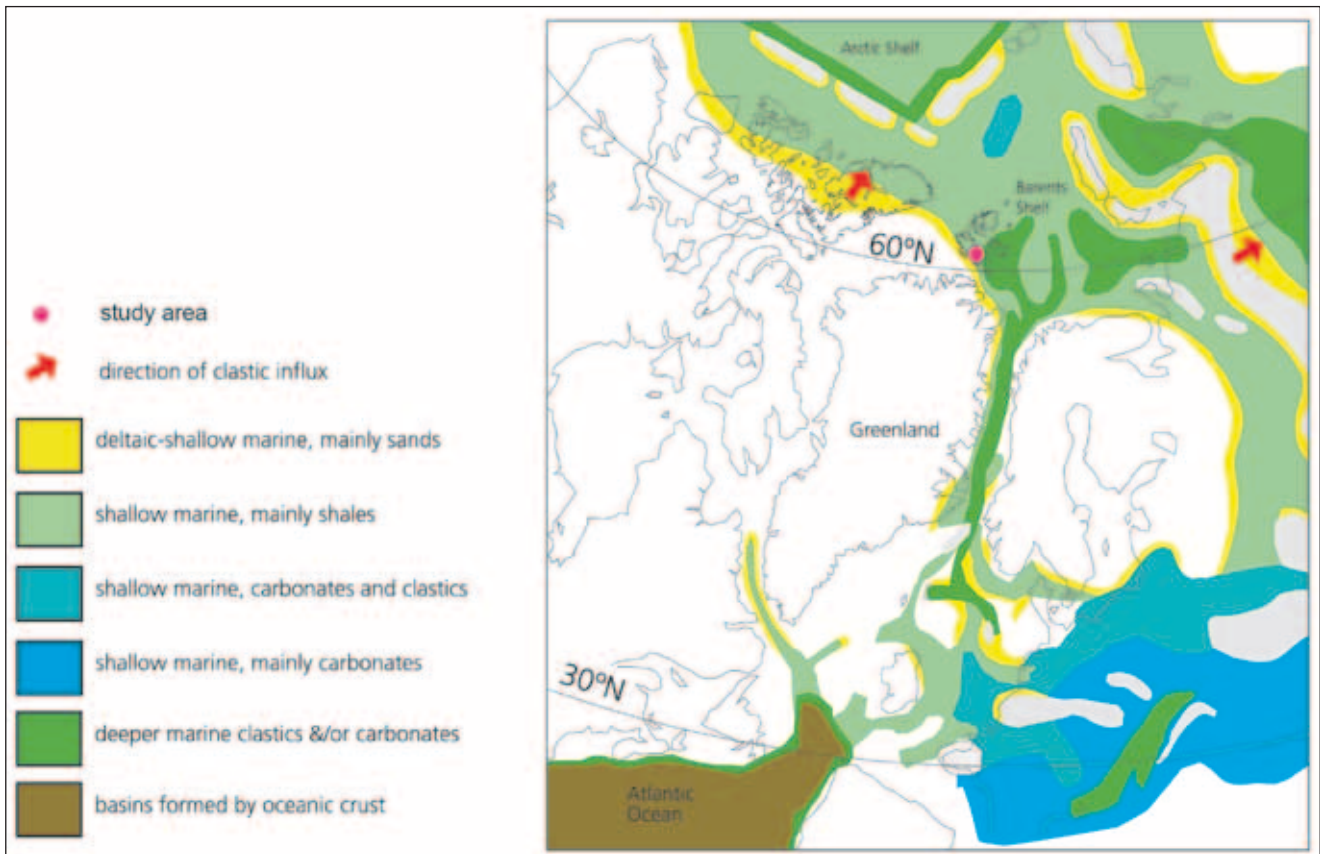
Figure 1. Paleogeographic map of the North Atlantic in the Late Jurassic (150 Ma) with the study area shown. Modified from Torsvik et al. (2002).
