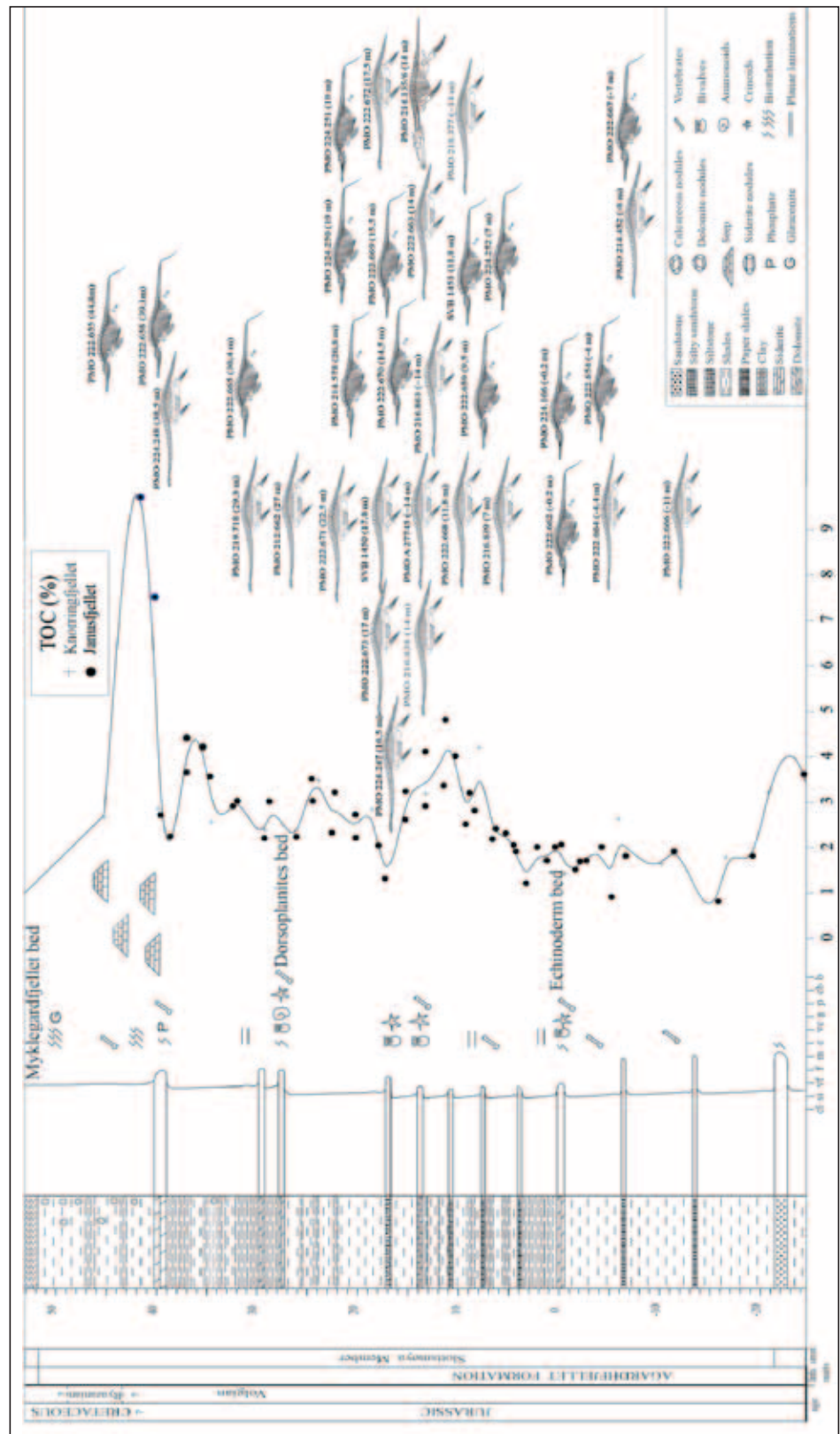
Figure 3. Stratigraphic scheme adapted from Novis (2012), Collignon & Hammer (this volume), Hammer et al. (this volume), Hammer et al. 2011 and Wierzbowski et al. (2011). Grain-size scales: b-boulders, c-coarse, cb-cobbles, cl-clay, f-fine, g-gravel, m-medium, p-pebbles, si-silt, vc-very coarse and vf-very fine.
