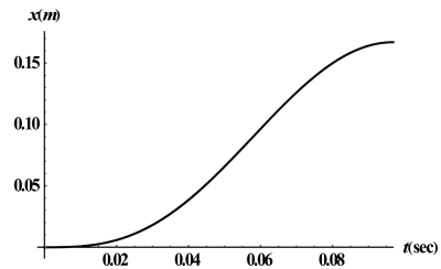
Figure 8. The variation of displacement versus time.
