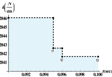
Figure 5. The variation of stiffness versus time.
