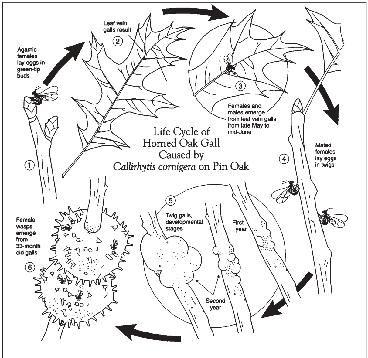
Figure 3. Life history of the horned oak gall wasp, C. cornigera , on pin oak as determined from research conducted in Lexington, Kentucky, 1996–1999. Illustration by Dennis Duross (Agricultural Communications Services, University of Kentucky).
