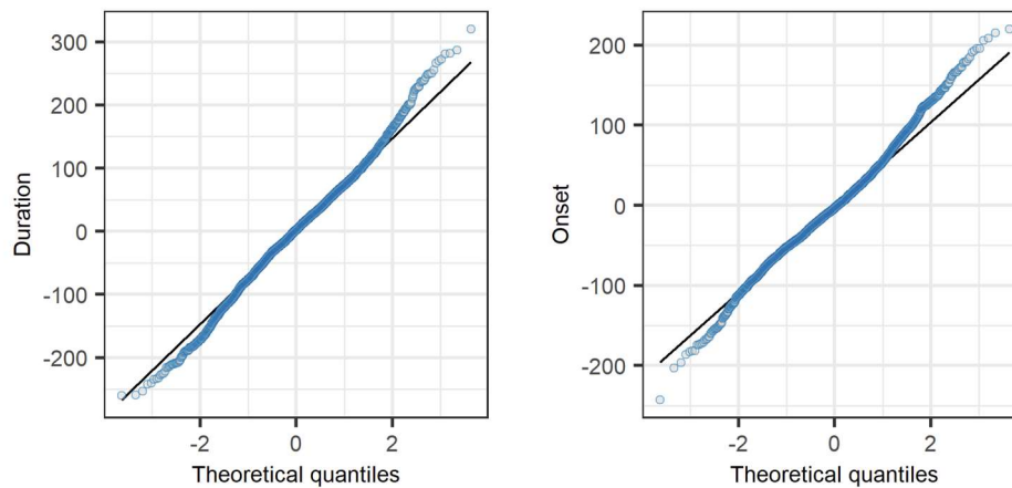
Figure S10. qq plots for the LMEMs presented in Table S2:
