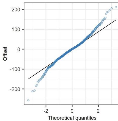
Figure S12. qq plot for the LMEM presented in Table S6.
