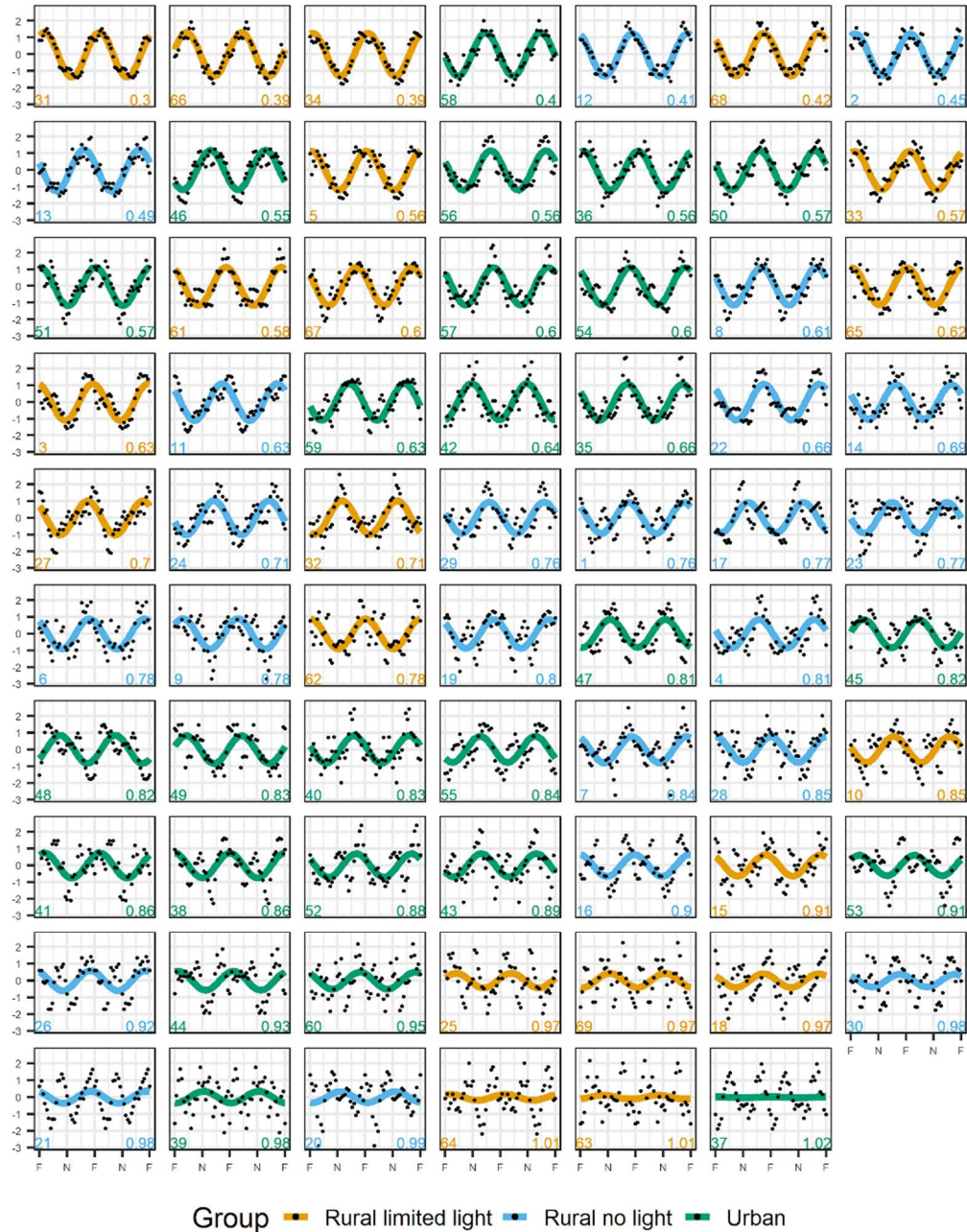
Figure S4. Individual patterns of sleep start times across the moon cycle. Double-plots of sleep onset expressed as z-scores of individual participants in the study across the moon cycle. Dots indicate the onset of sleep on each night in the cycle, and colored lines represent the best fit of a sine wave with a 30-days period through a non-linear least squares approach. The number on the bottom left of each plot identifies the participant and the one on the bottom right the standard error of the regression (S). The data correspond to participants with records for at least 80% of the moon cycle. Participants are ordered from best to worst fits as evaluated by S: minimum = 0.30, median = 0.78, maximum = 1.02. F = full moon, N = new moon.
