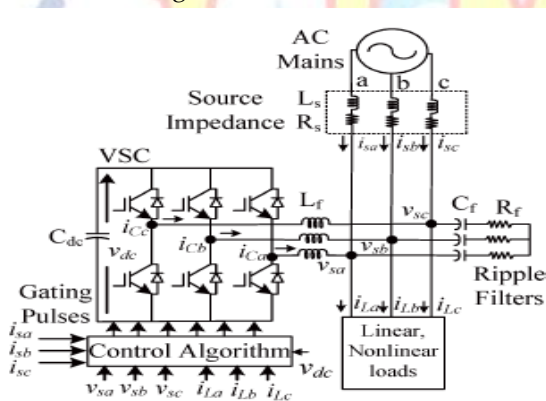
Figure 4 Schematic diagram of VSC-based DSTATCOM.
