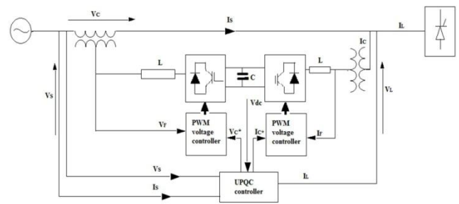
Figure 4: Basic Configuration of UPQC
