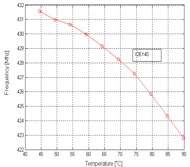
Frequency response of one sensor (X26Y40) with constant voltage core (1.0 V)
