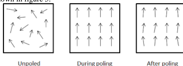
Figure 1. Alignments of Dipoles in a Piezoelectric Material
