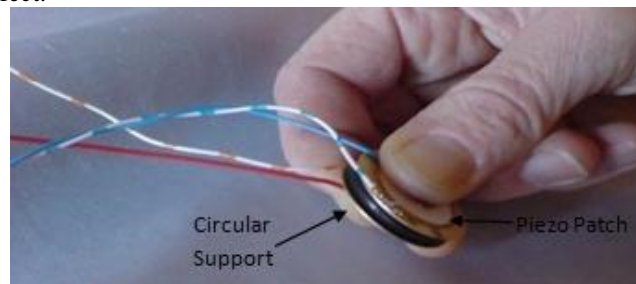
Figure 4. Piezoelectric Disk with circular support Generates Voltage under Deformation
