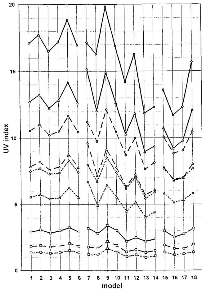
Figure 1. Ultraviolet index calculated with models 1–18 (see text for details) for solar zenith angles: 15° ( \diamond ), 30° ( \Delta ) and 60° ( \square ) and for total ozone: 190 DU (—), 285 DU (---) and 380 DU (.....). Other parameters: surface at sea level, albedo: 0.03, aerosol with optical depth 0.6 and single scattering albedo 0.92 at 340 nm.
