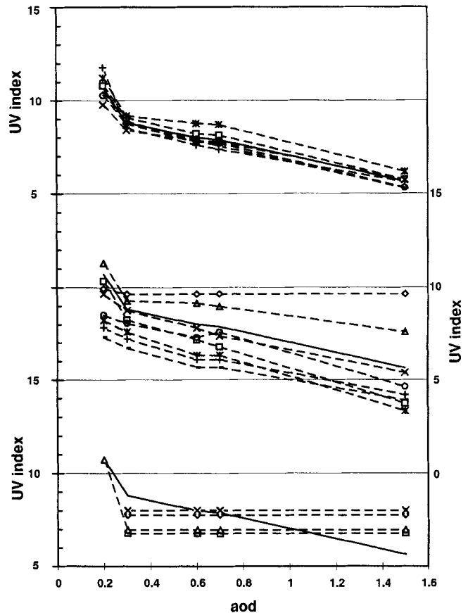
Figure 2. Ultraviolet index as function of aerosol load for solar zenith angle 30°, total ozone content 285 DU and albedo 0.03. The aod values indicate aerosol optical depth at 340 nm and are relevant also for the single scattering albedo, which is varied simultaneously (see text). For aod 0.3, 0.6 and 1.5, the other atmospheric properties are taken with values that are valid at sea level. For aod 0.2 all atmospheric parameter values are appropriate for a surface at 2000 m above sea level. Results of the three model groups are separated by 10 UV index values against each other. In each group values of reference UV index (arithmetic mean of results of models 1–6) are given as solid lines. Upper part, left axis, multiple-scattering models with symbols: 1, –; 2, \square ; 3, +; 4, \times ; 5, \star ; 6, \circ ; middle part, right axis, fast spectral models with symbols: 7, \diamond ; 8, \square ; 9, \Delta ; 10, \times ; 11, \star ; 12, \circ ; 13, –; 14, +; lower part, left axis, empirical models with symbols: 15, \diamond ; 16, \square ; 17, \Delta ; 18, \times .
