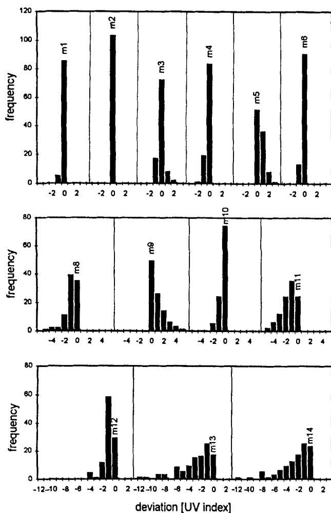
Figure 4. Histograms of absolute UV index deviations as differences between modeled and reference UV index. Model number is given in each case at value 0. Columns contain \pm 0.5 UV index values around the value marked.
