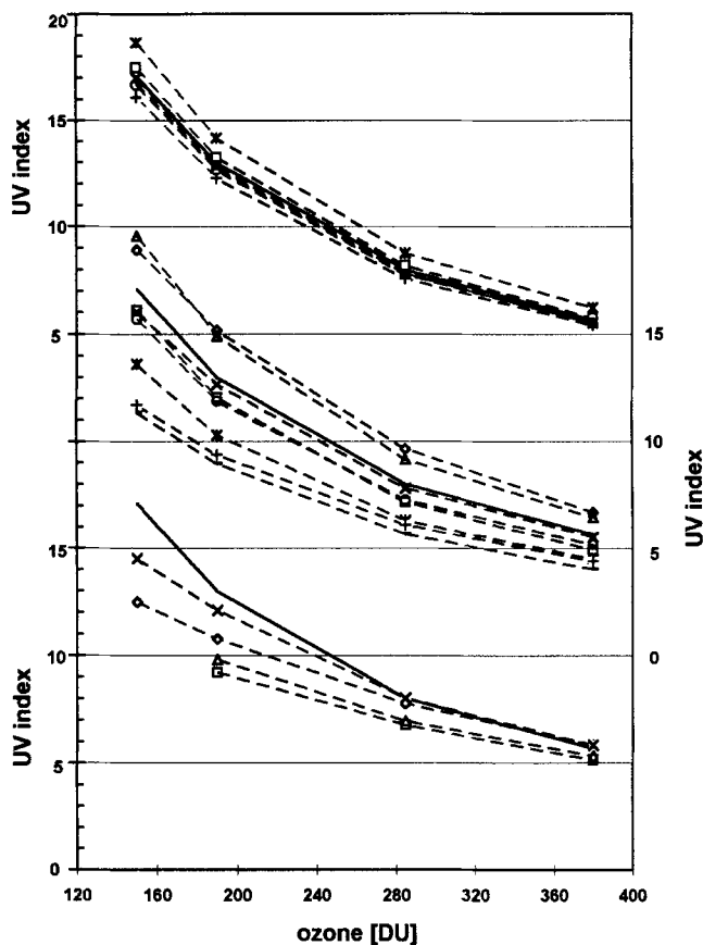
Figure 3. Ultraviolet index as a function of total ozone content for solar zenith angle 30°, aerosol with aod 0.6 and single scattering albedo 0.92 at 340 nm and albedo 0.03. Results of the three model groups are separated by 10 UV index values against each other. In each group values of the reference UV index are given as solid lines. Upper part, left axis, multiple-scattering models with symbols: 1, -; 2, □; 3, +; 4, ×; 5, ★; 6, ○; middle part, right axis, fast spectral models with symbols: 7, ◇; 8, □; 9, △; 10, ×; 11, ★; 12, ○; 13, -; 14, +; lower part, left axis, empirical models with symbols: 15, ◇; 16, □; 17, △; 18, ×.
