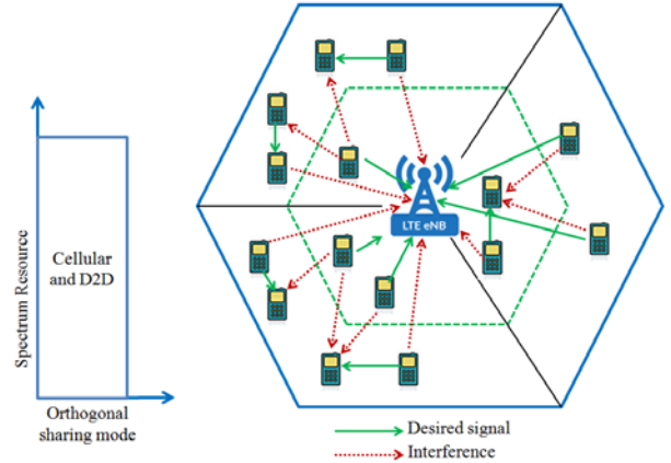
Fig. 2. (a) Uplink resource sharing mode; (b) Interference scenario for D2D communication in an uplink cellular network.
