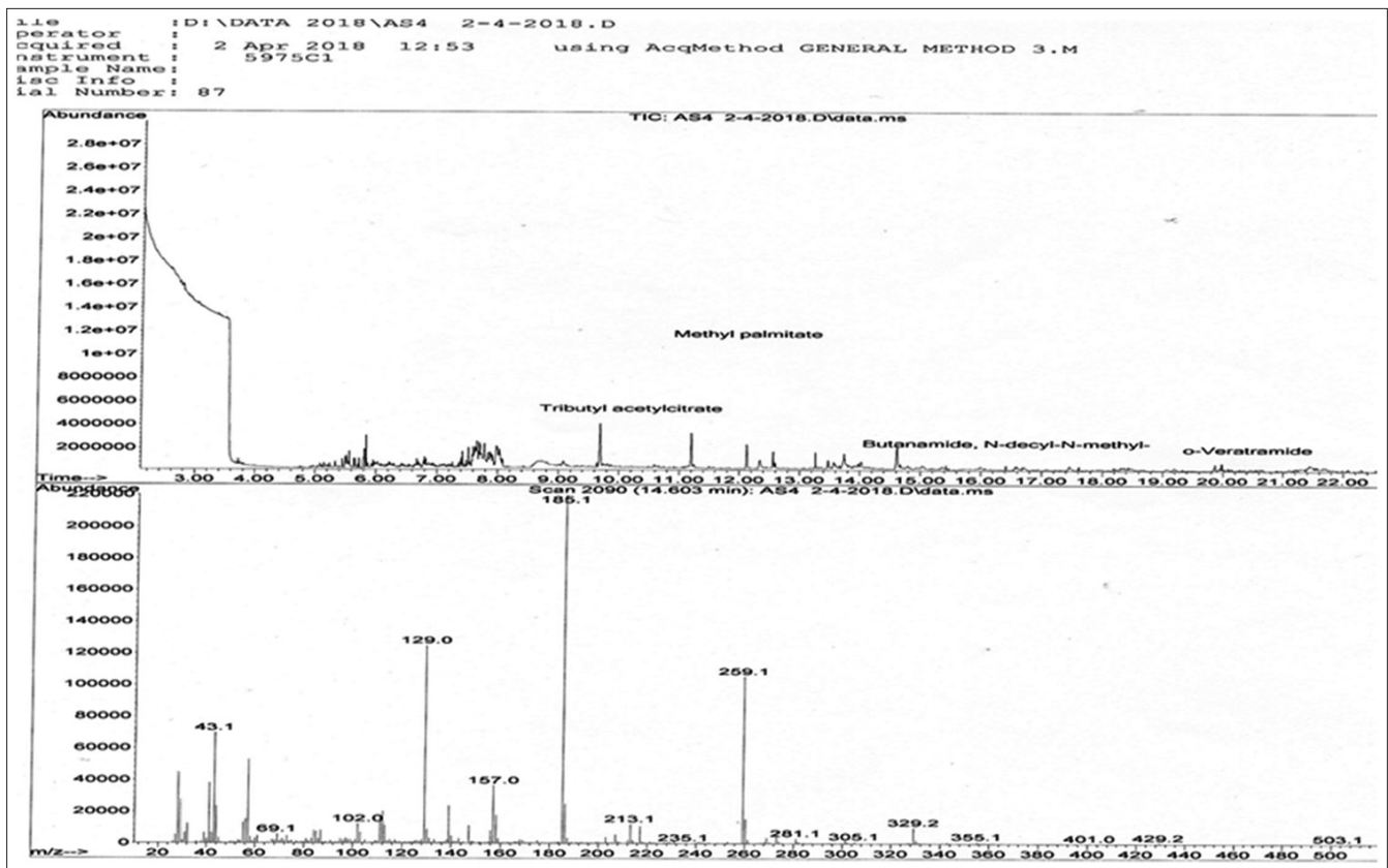
Figure 4: Gas chromatography-mass spectrum for four compound in aquatic layer
