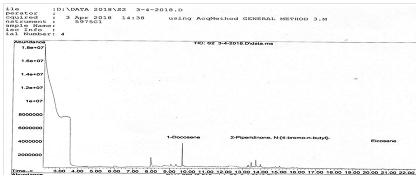
Figure 2: Gas chromatography–mass spectrometry for three compounds in organic layer
