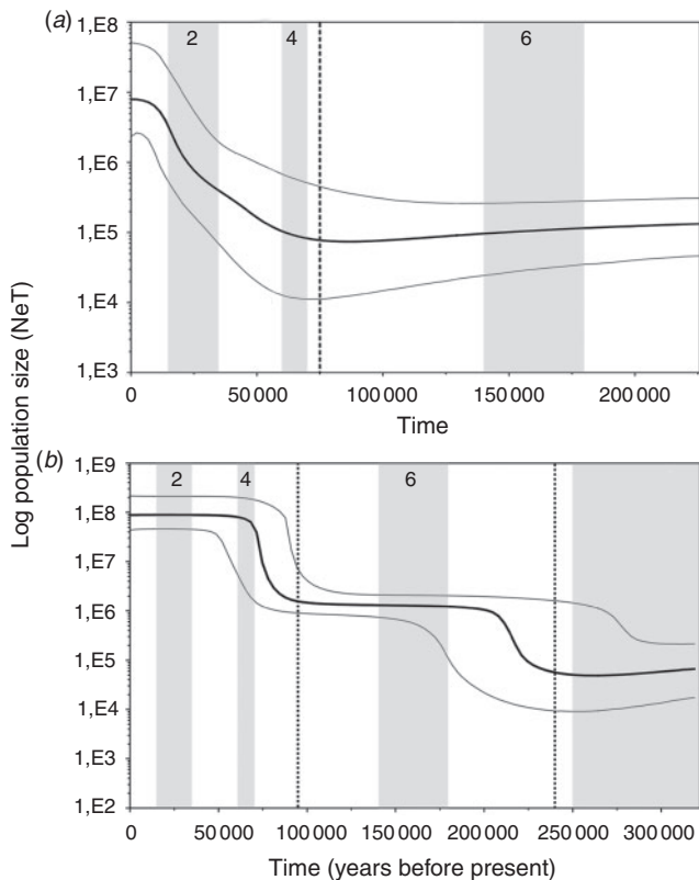
Fig. 3. Bayesian Skyline Plots for the (a) COI gene and (b) control region of Scyllarides brasiliensis . The maximum time is the upper 95% HPD of the root height. The median estimate (black solid line) and 95% HPD limits (grey solid line) are indicated. Dotted lines correspond to the approximate onset of the expansion events. The main glaciations over the last 250 000 years are shaded in grey: MIS6 (180–140 000 years ago), MIS4 (70–60 000 years ago) and MIS2 (35–15 000 years ago) (Gibbard and Cohen 2009).
