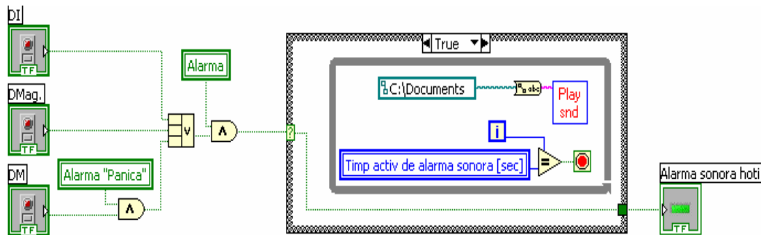
Figure 3: Diagram with acoustical alarm
