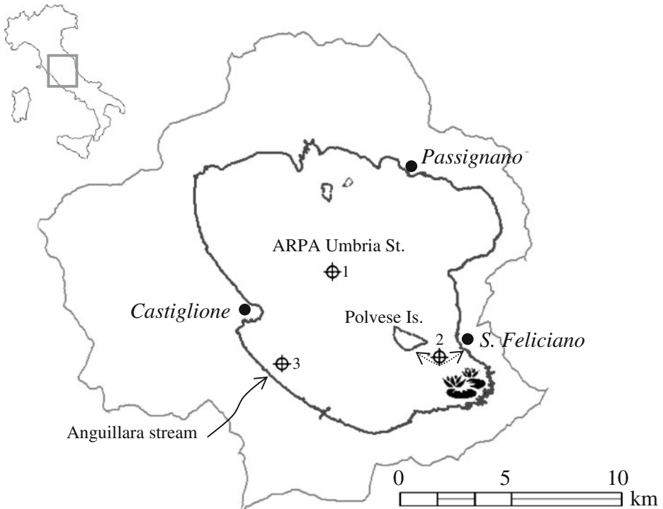
Fig. 1 The figure shows Lake Trasimeno location (central Italy) with its small catchment basin. The positions of the pelagic station sampled by ARPA Umbria (nr. 1) is indicated together with other two stations (i.e., nr. 2 and 3) used in this study to investigate water quality trends. The substrates in the southern-eastern bottom of the lake are colonised by wide extensions of macrophytes (indicated by an icon). The lake has no tributary but is fed by small streams (the one with the highest flows is Anguillara). The dotted line with two arrows indicate the ferry route from S. Feliciano to Polvese Island
